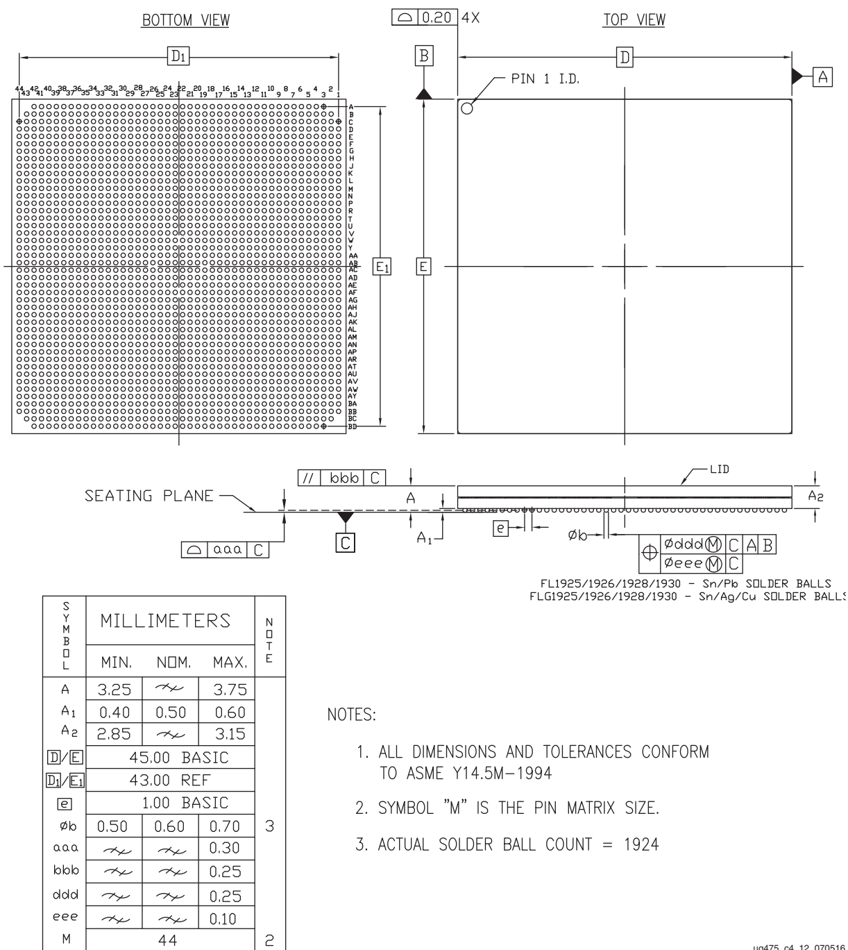
Figure 4-45: FL1925, FLG1925, FL1926, FLG1926, FL1928, FLG1928, and FL1930, FLG1930 Flip-Chip BGA Package Specification for Virtex-7 FPGAs
