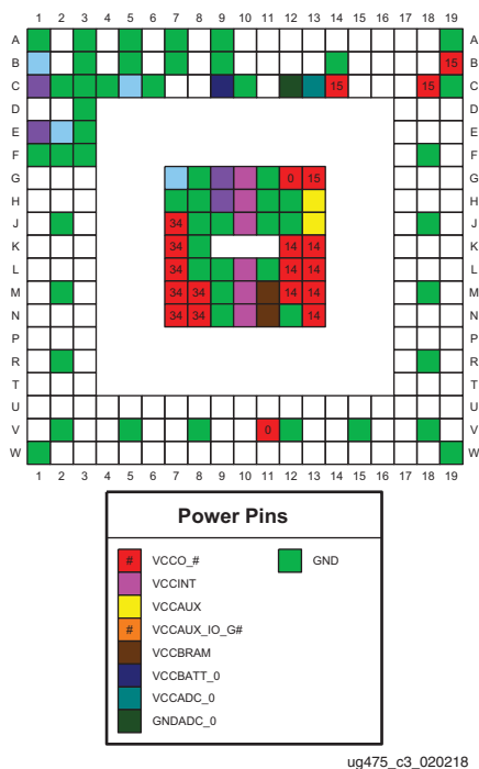
Figure 3-48: CPG238 Package—XC7A12T, XC7A25T, XA7A12T, and XA7A25T Power and GND Placement
