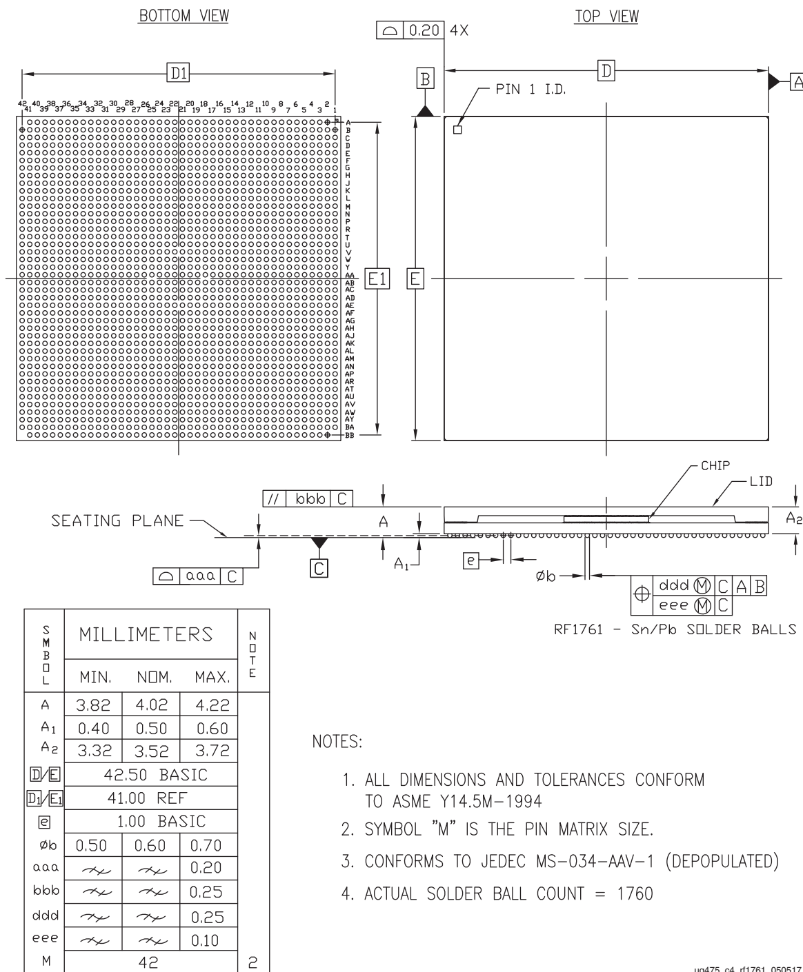
Figure 4-47: RF1761 Flip-Chip BGA Package Specifications for Virtex-7 FPGAs
