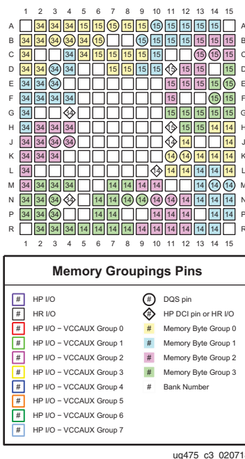
Figure 3-19: CSGA225 Package—XC7S25 and XA7S25 Memory Groupings
