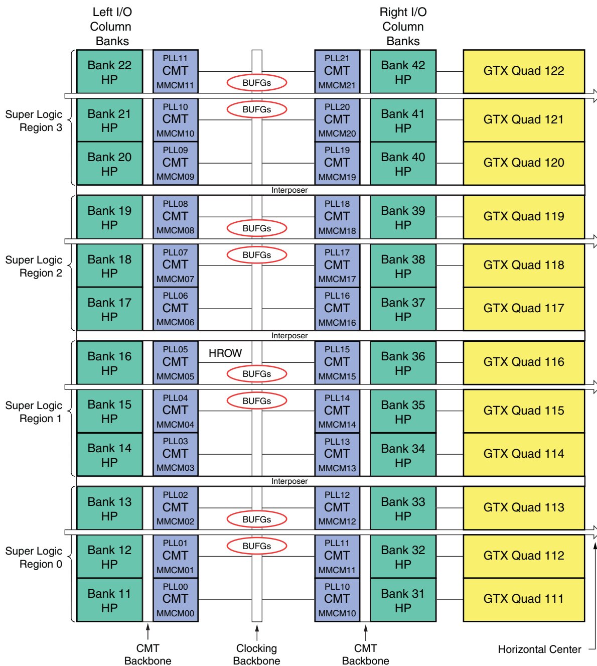
Figure 1-19: XC7V2000T Banks
