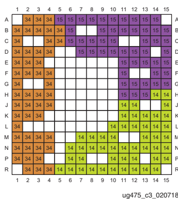
Figure 3-18: CSGA225 Package—XC7S25 and XA7S25 I/O Banks
