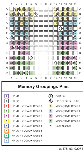
Figure 3-7: FTGB196 Package—XC7S6 and XC7S15 Memory Groupings
