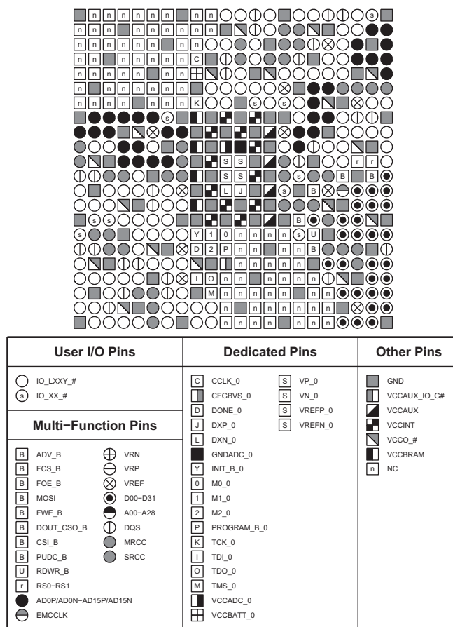
Figure 3-29: FGGA484 Package—XC7S50 and XA7S50 Pinout Diagram
