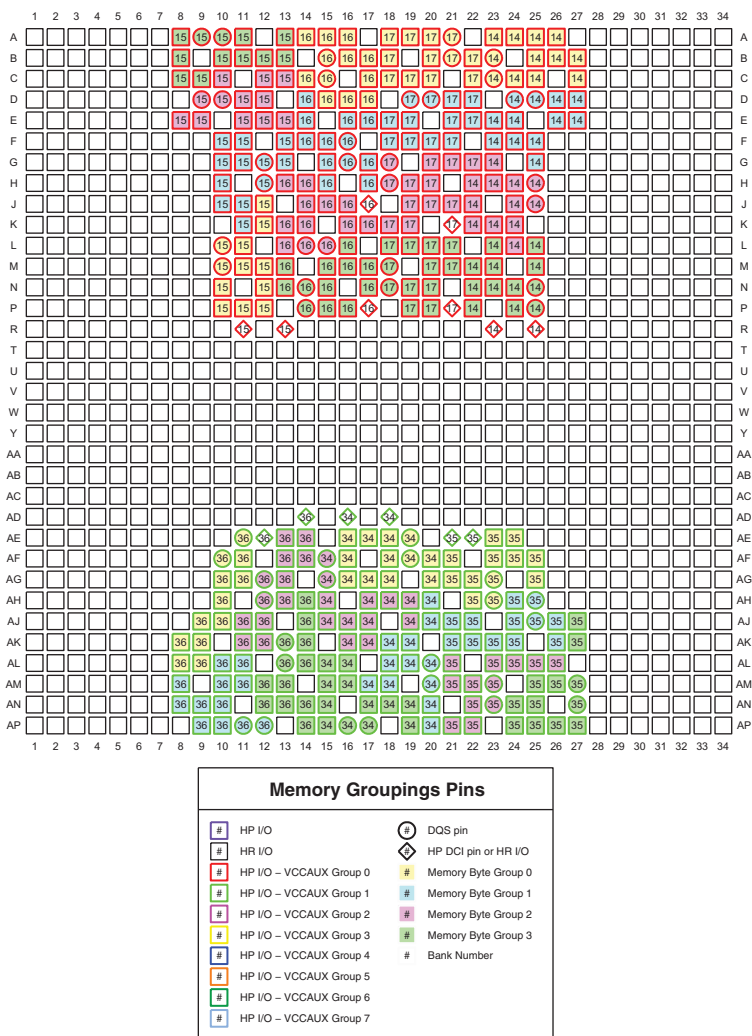
Figure 3-159: FF1158, FFG1158, FFG1158, and RF1158 Packages—XC7VX415T, XC7VX550T, and XC7VX690T Memory Groupings
