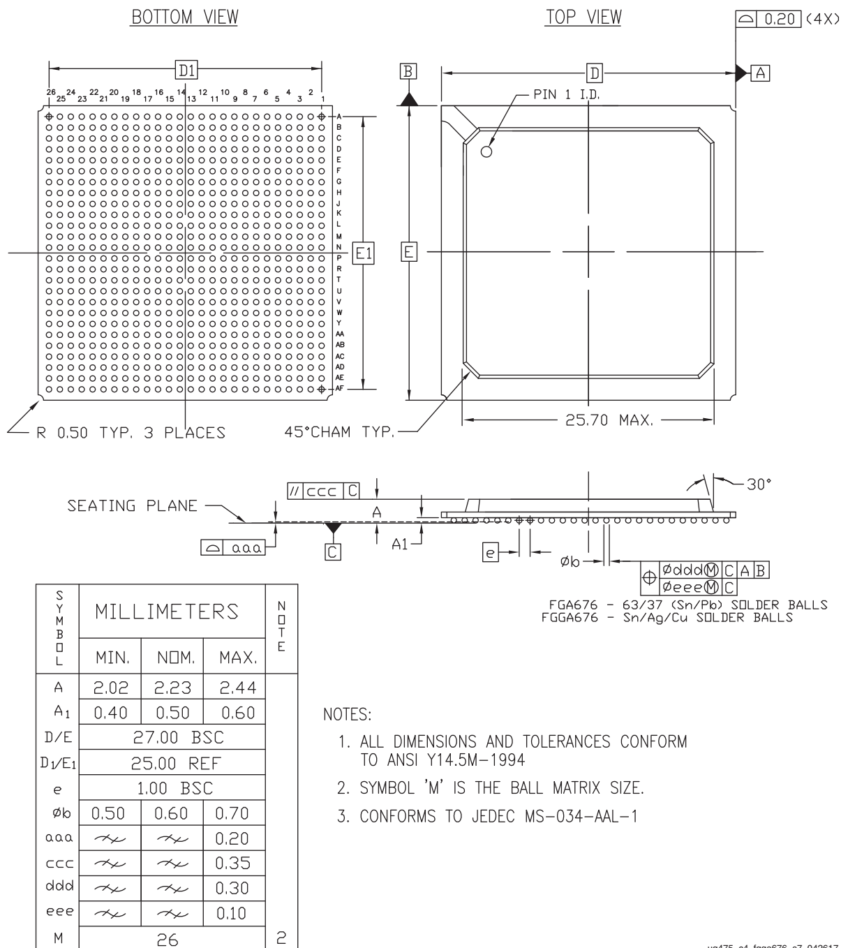
Figure 4-6: FGGA676 Wire-bond Fine-Pitch BGA Package Specification for Spartan-7 FPGAs
