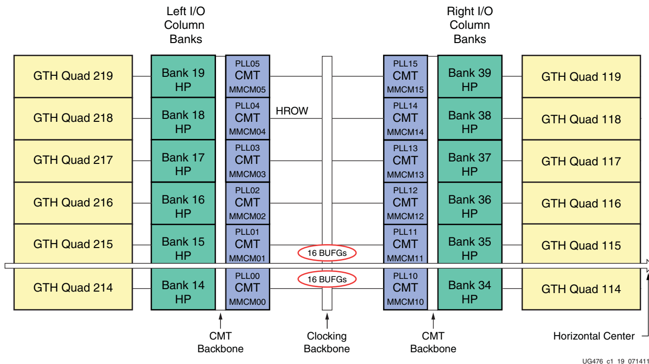
Figure 1-21: XC7VX415T Banks
