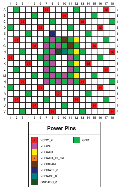
Figure 3-52: CS324 and CSG324 Packages—XC7A15T, XC7A35T, XC7A50T, XC7A75T, and XC7A100T CSG324 Packages (only)—XA7A15T, XA7A35T, XA7A50T, XA7A75T, and XA7A100T Power and GND Placement
