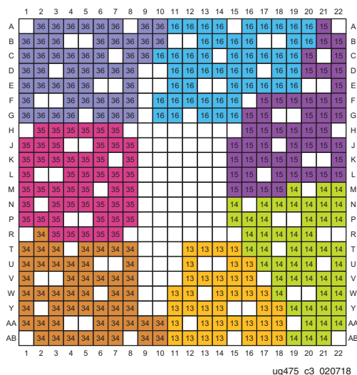
Figure 3-34: FGGA484 Package—XC7S75, XC7S100, XA7S75, and XA7S100 I/O Banks
