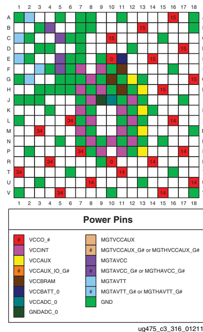
Figure 3-64: CS325 and CSG325 Packages—XC7A15T, XC7A35T, and XC7A50T CSG325 Packages (only)—XA7A15T, XA7A35T, and XA7A50T Power and GND Placement
