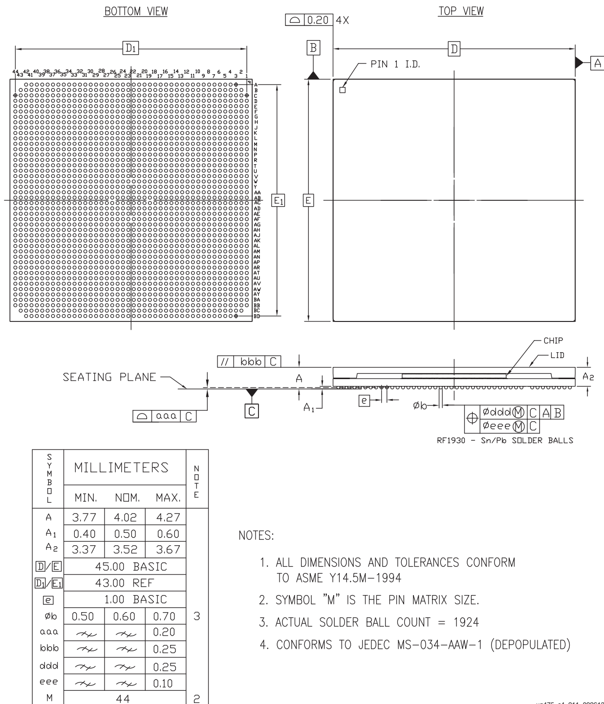
Figure 4-48: RF1930 Flip-Chip BGA Package Specifications for Virtex-7 FPGAs
