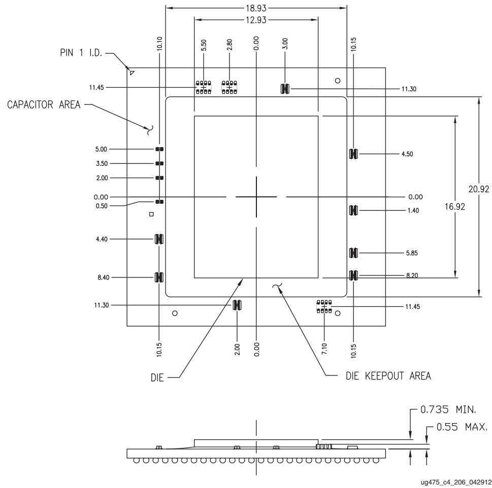
Figure 4-29: XC7K410T FBG676, FBG676, and FBV676 Die Dimensions with Capacitor Locations
