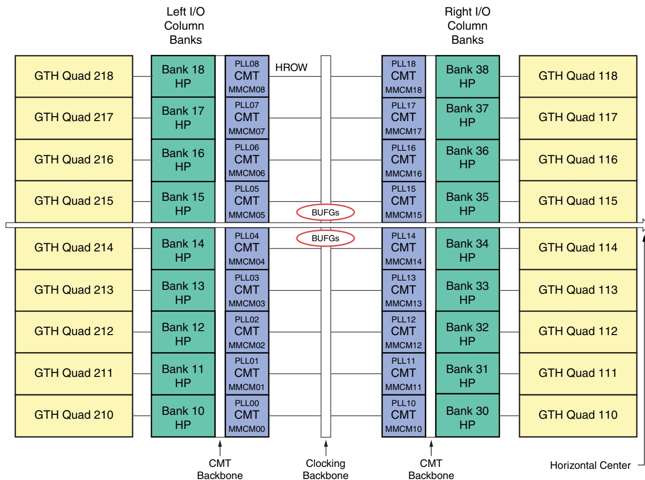
Figure 1-25: XC7VX980T and XQ7VX980T Banks
