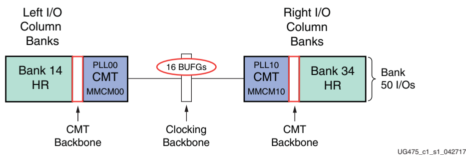
Figure 1-1: XC7S6, XA7S6, XC7S15, and XA7S15 Banks
