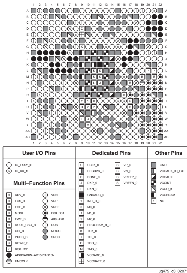
Figure 3-33: FGGA484 Package—XC7S75, XC7S100, XA7S75, and XA7S100 Pinout Diagram
