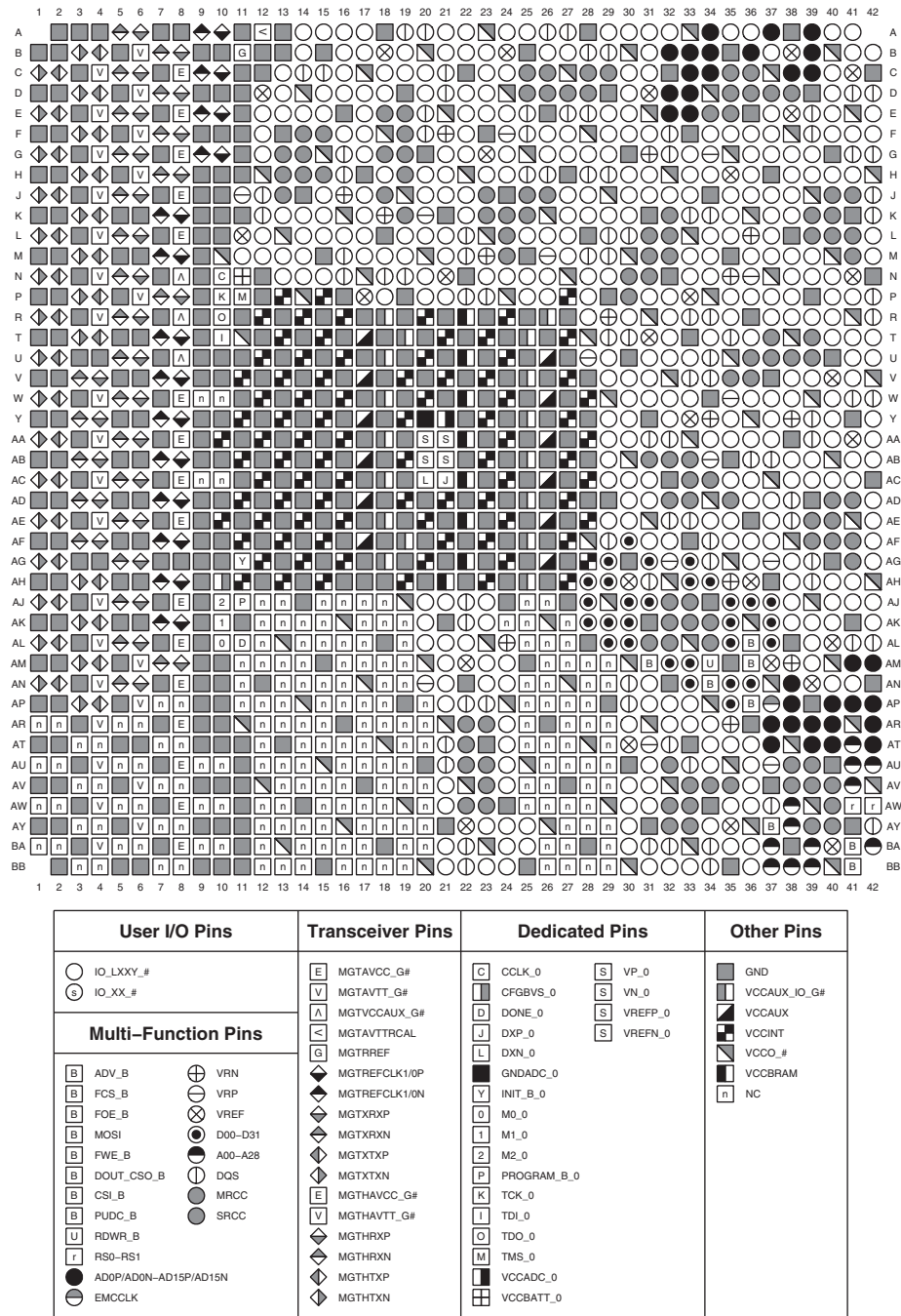
Figure 3-173: FF1761, FFG1761, and RF1761 Packages—XC7VX485T Pinout Diagram
