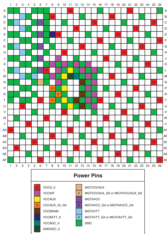
Figure 3-116: FF676, FFG676, FFF676, and RF676 Packages—XC7K160T, XA7K160T, XC7K325T, and XC7K410T Power and GND Placement
