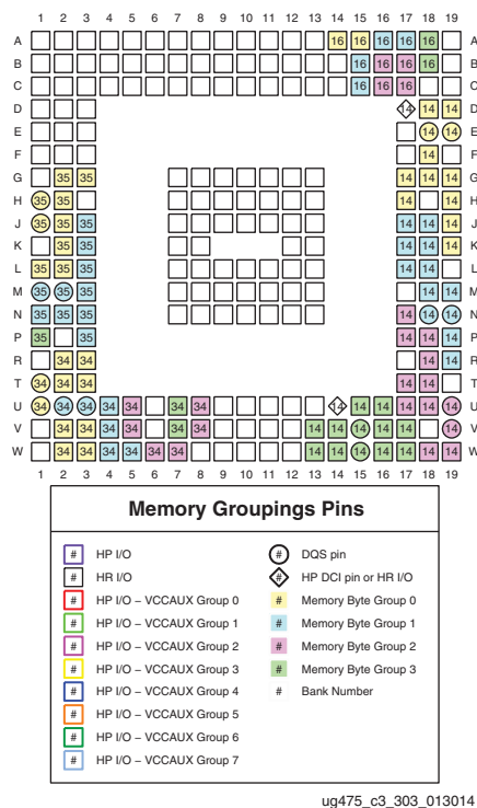
Figure 3-43: CP236 and CPG236 Packages—XC7A15T, XC7A35T, and XC7A50T CPG236 Packages (only)—XA7A15T, XA7A35T, and XA7A50T Memory Groupings
