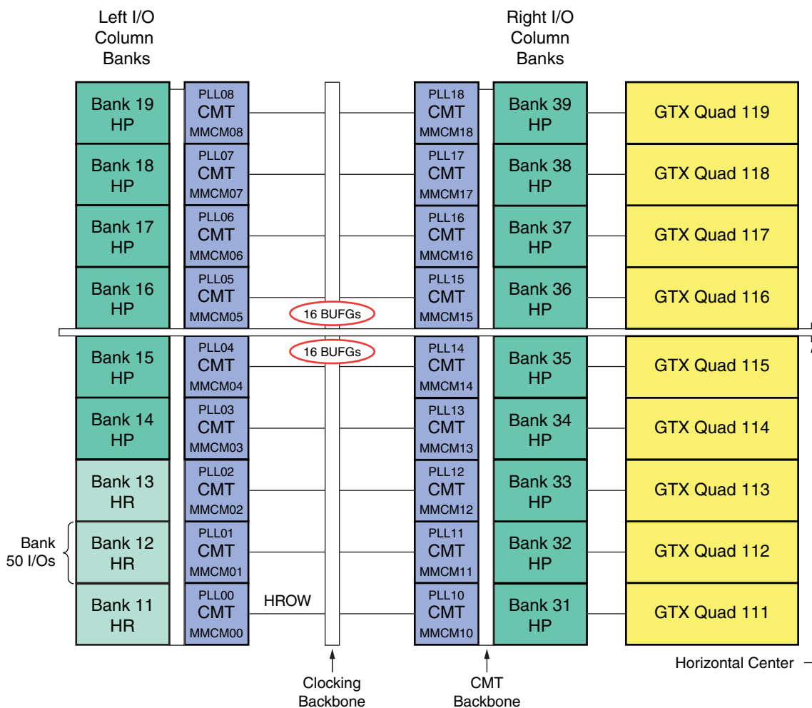
Figure 1-18: XC7V585T and XQ7V585T Banks
