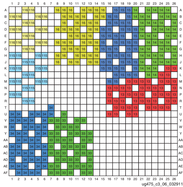
Figure 3-102: FB676, FBG676, and FBV676 Packages—XC7K70T I/O Banks
