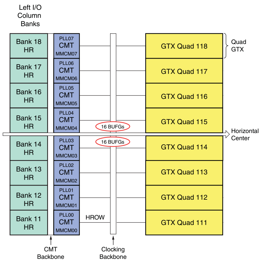
Figure 1-16: XC7K420T Banks
