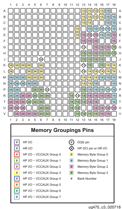
Figure 3-23: CSGA324 Package—XC7S25 and XA7S25 Memory Groupings
