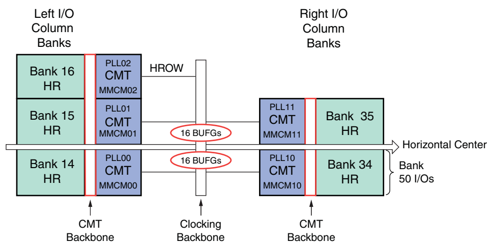
Figure 1-3: XC7S50 and XA7S50 Banks
