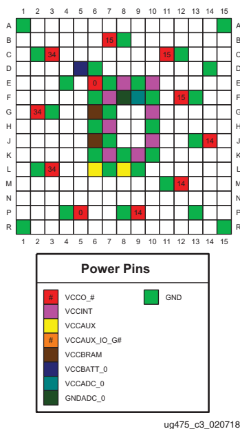
Figure 3-20: CSGA225 Package—XC7S25 and XA7S25 Power and GND Placement
