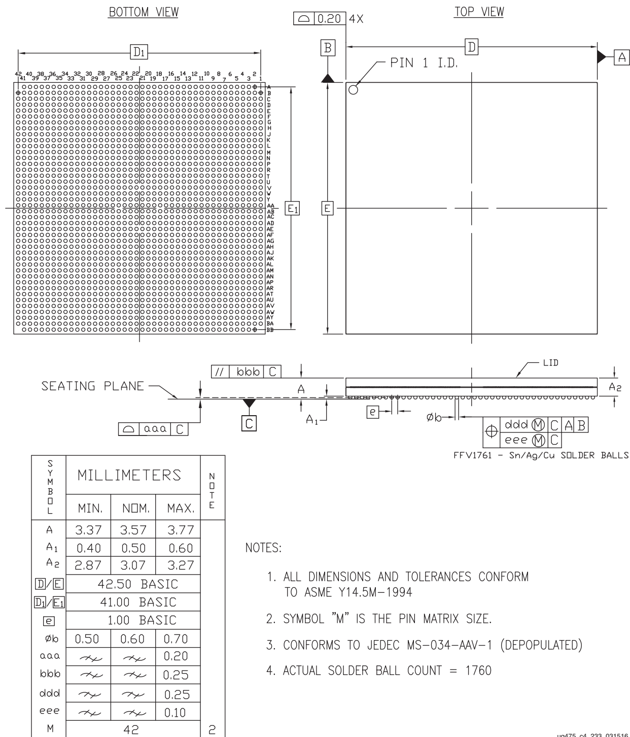
Figure 4-42: FFV1761 Flip-Chip BGA Package Specification for Virtex-7 FPGAs
