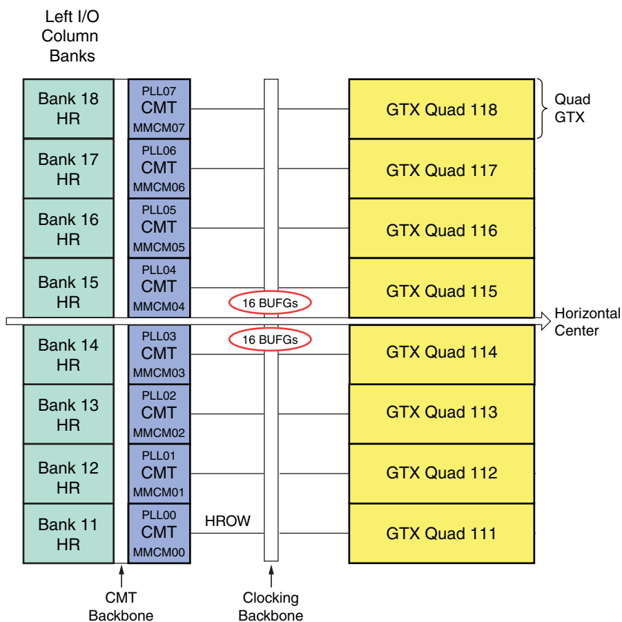
Figure 1-17: XC7K480T Banks
