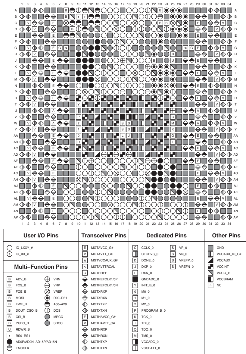
Figure 3-157: FF1158, FFG1158, FFV1158, and RF1158 Packages—XC7VX415T, XC7VX550T, and XC7VX690T Pinout Diagram
