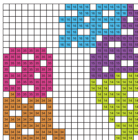
Figure 3-30: FGGA484 Package—XC7S50 and XA7S50 I/O Banks
