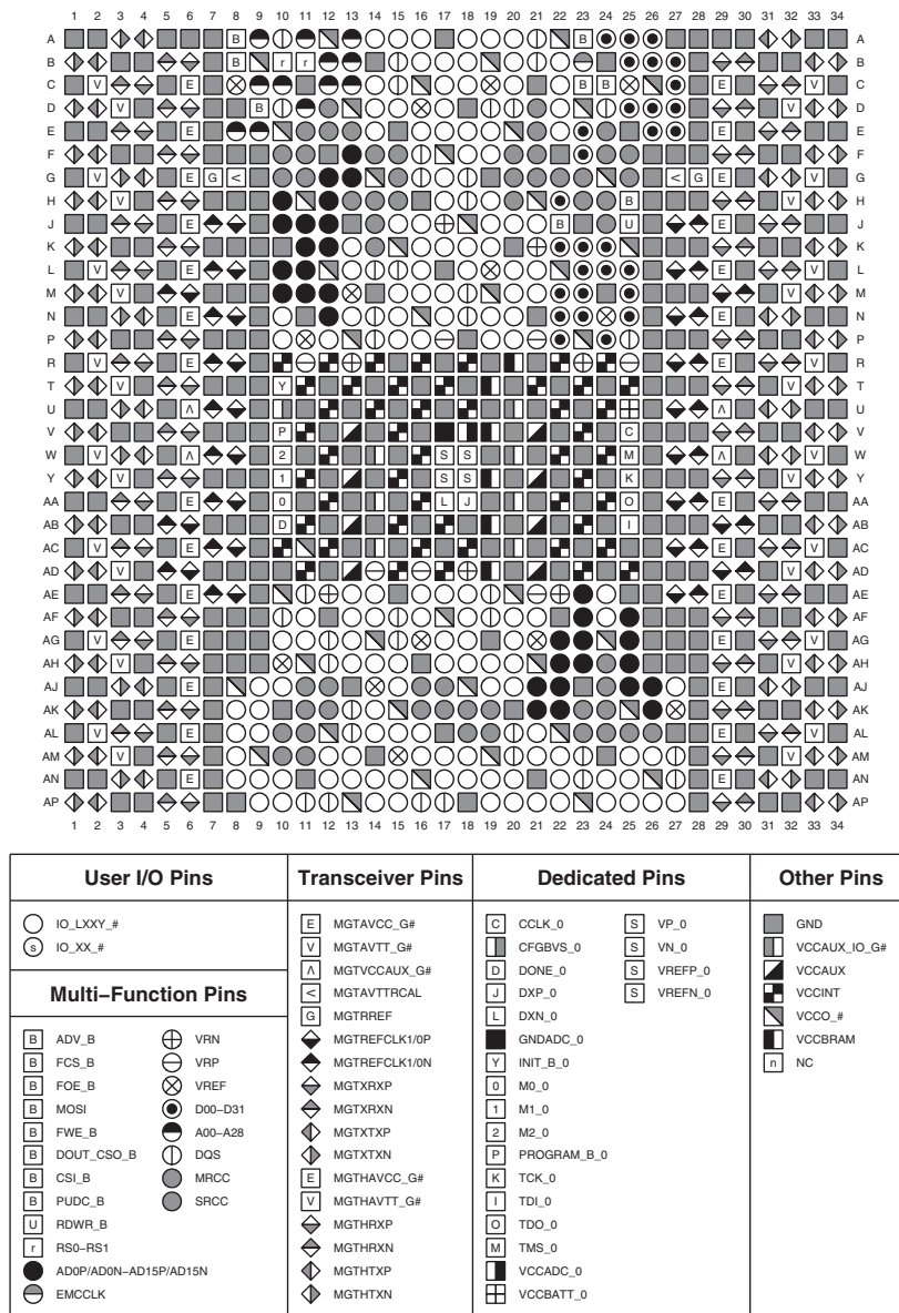
Figure 3-169: FF1158, FFG1158, and FFV1158 Packages—XC7VX485T Pinout Diagram
