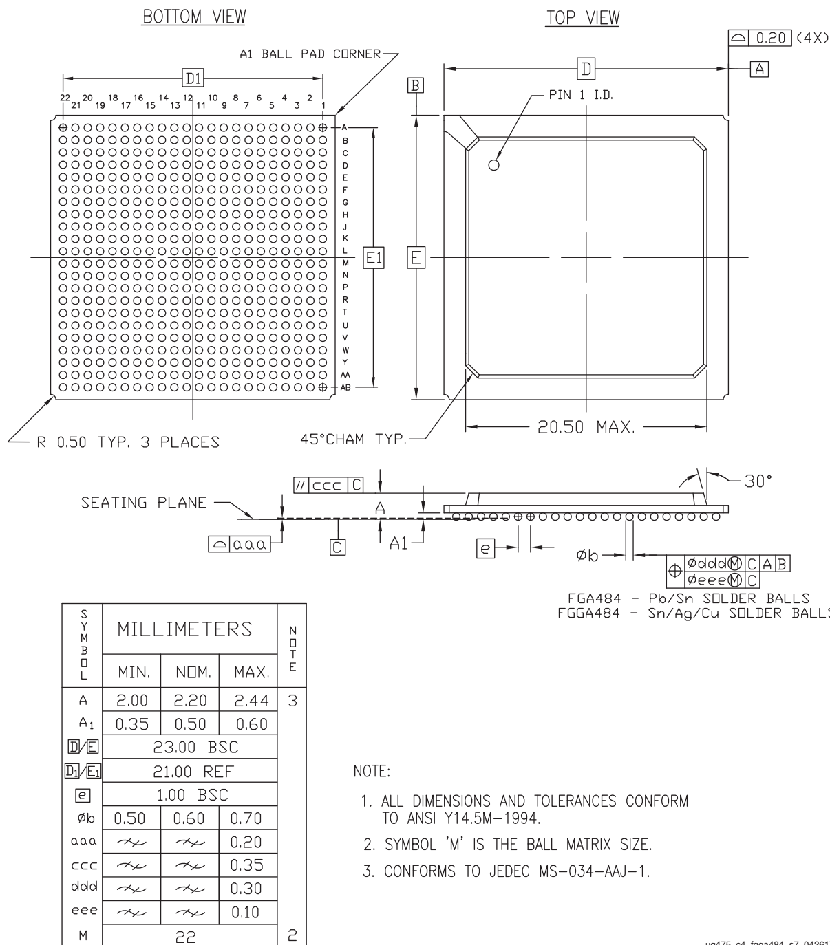
Figure 4-5: FGGA484 Wire-bond Fine-Pitch BGA Package Specification for Spartan-7 FPGAs
