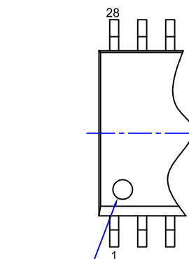
PIN #1 INDICATOR OPTION 3 PIN 1 ONLY
