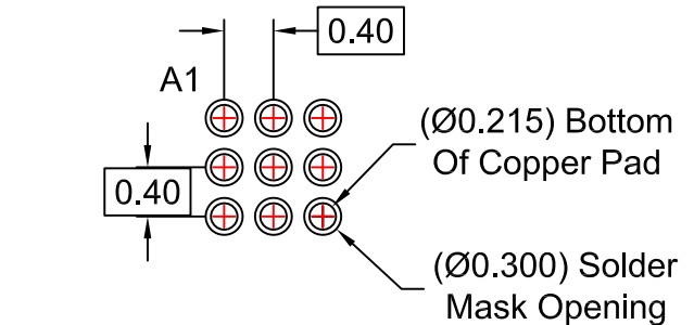
RECOMMENDED LAND PATTERN (NSMD PAD TYPE)
