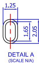
LAND PATTERN RECOMMENDATIONS
