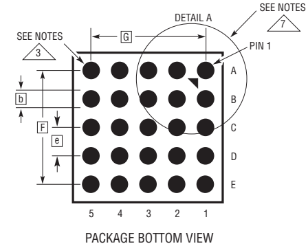
PACKAGE BOTTOM VIEW
