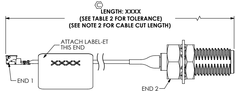
FIG 1 MHXXX-MH1RP-01BJ1-XXXX SHOWN
