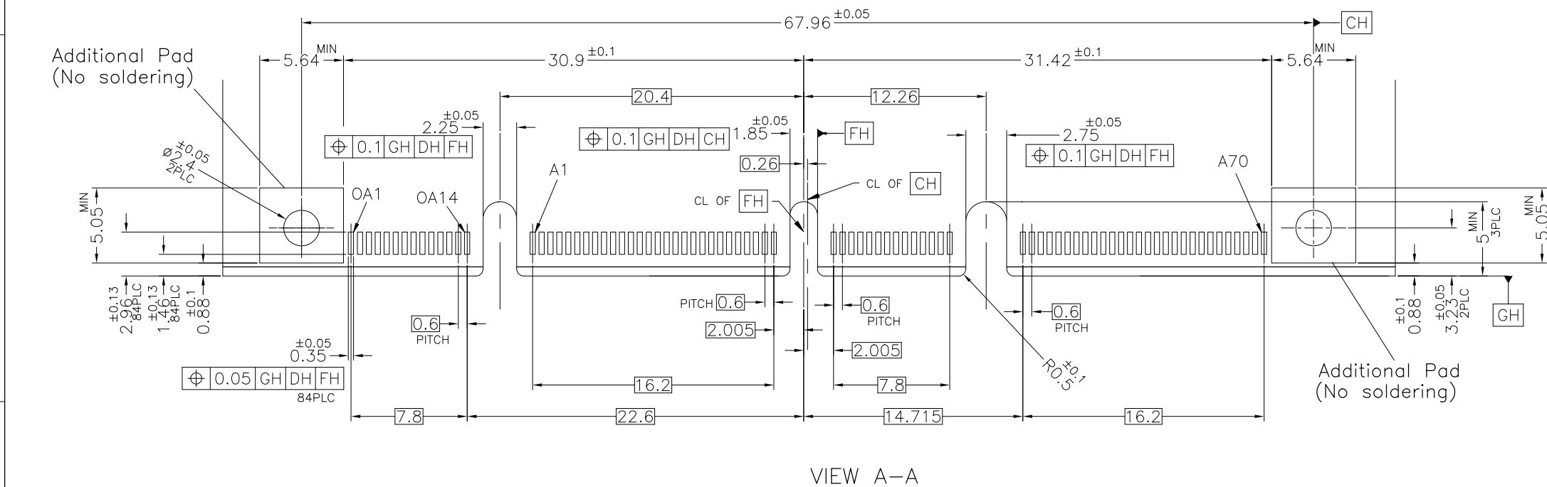
HOST BOARD LAYOUT FOR HVM
