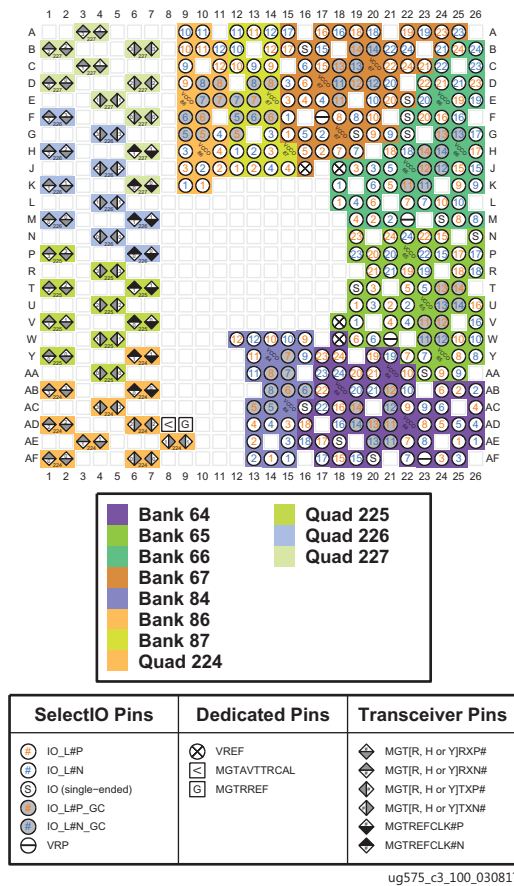
Figure 3-79: FFVB676 Package—XCKU3P and XCKU5P and FFRB676 Package—XQKU5P I/O Bank Diagram
