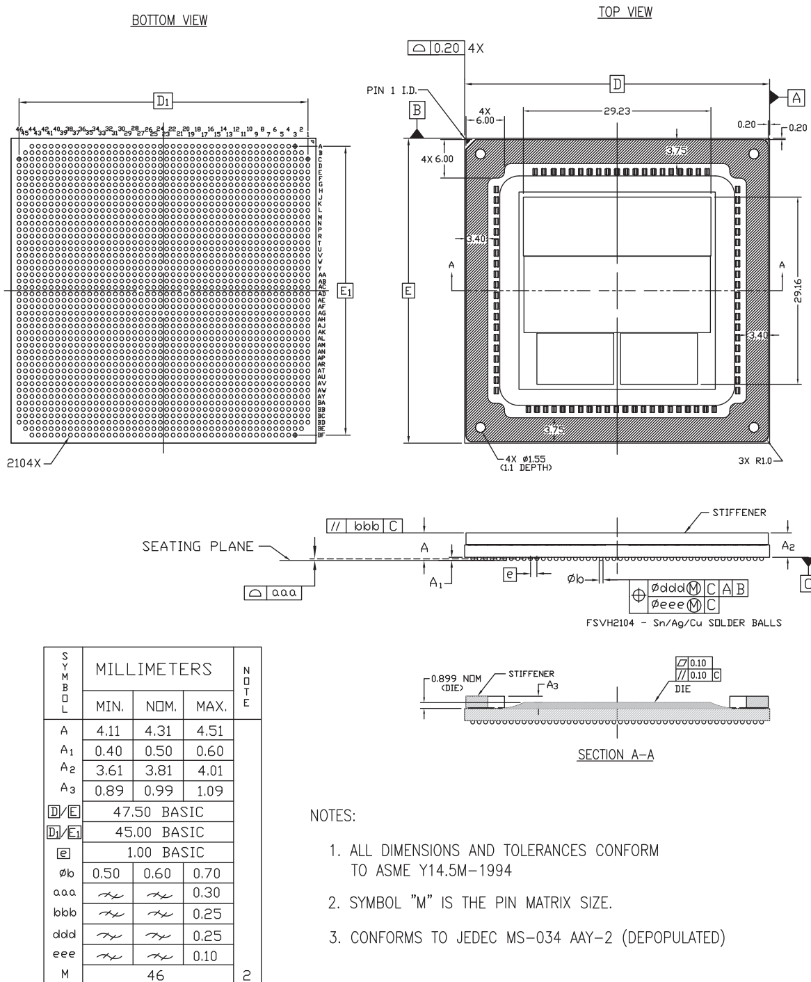
Figure 4-49: Package Dimensions for FSVH2104 (XCVU35P and XCVU45P)
