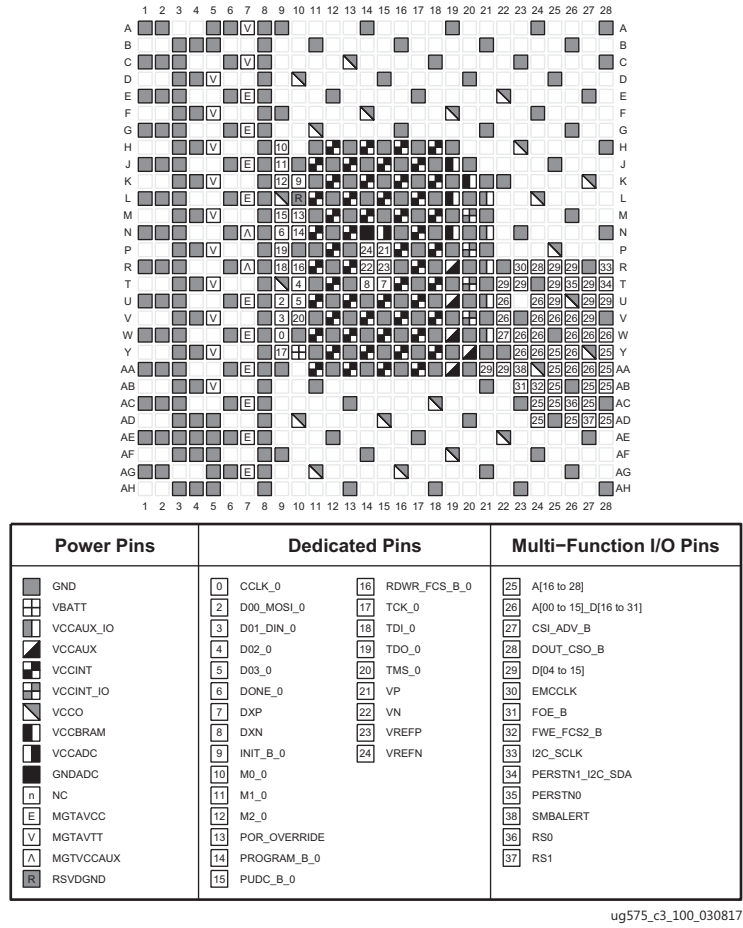
Figure 3-82: SFVB784 Package—XCKU3P and XCKU5P and SFRB784 Package—XQKU5P Configuration/Power Diagram
