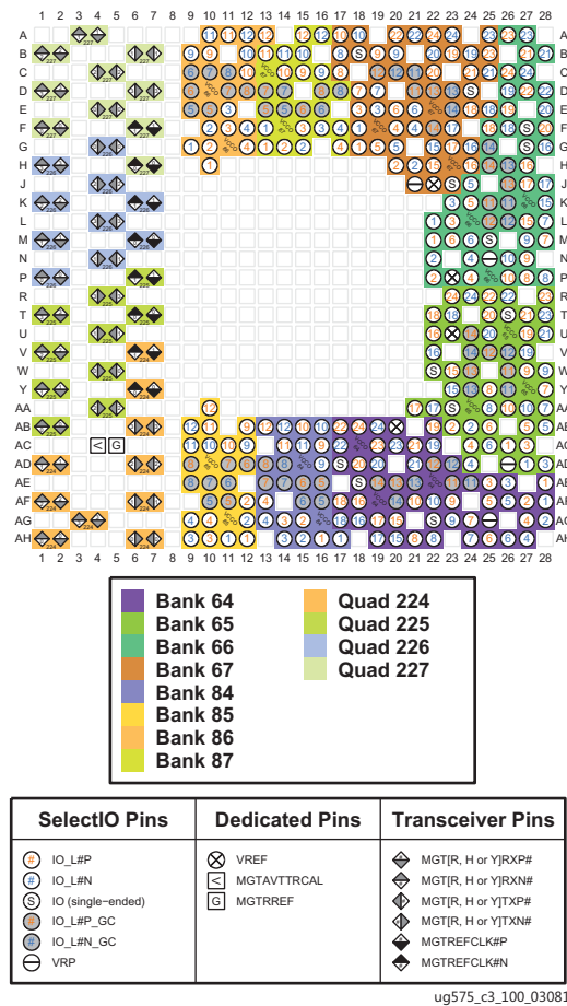
Figure 3-81: SFVB784 Package—XCKU3P and XCKU5P and SFRB784 Package—XQKU5P I/O Bank Diagram
