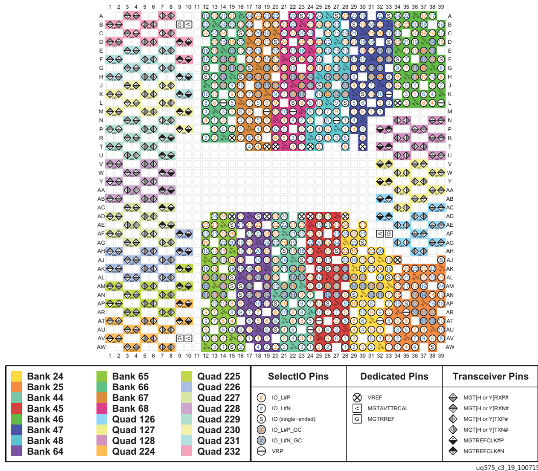
Figure 3-19: FLVA1517 Package—XCKU085 and XCKU115 I/O Bank Diagram
