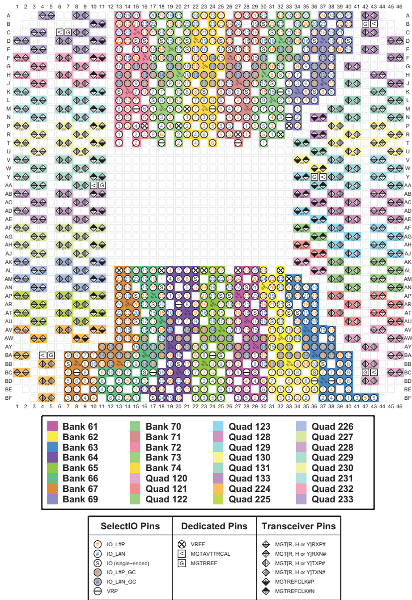
Figure 3-135: FIGD2104 Package—XCVU13P I/O Bank Diagram
