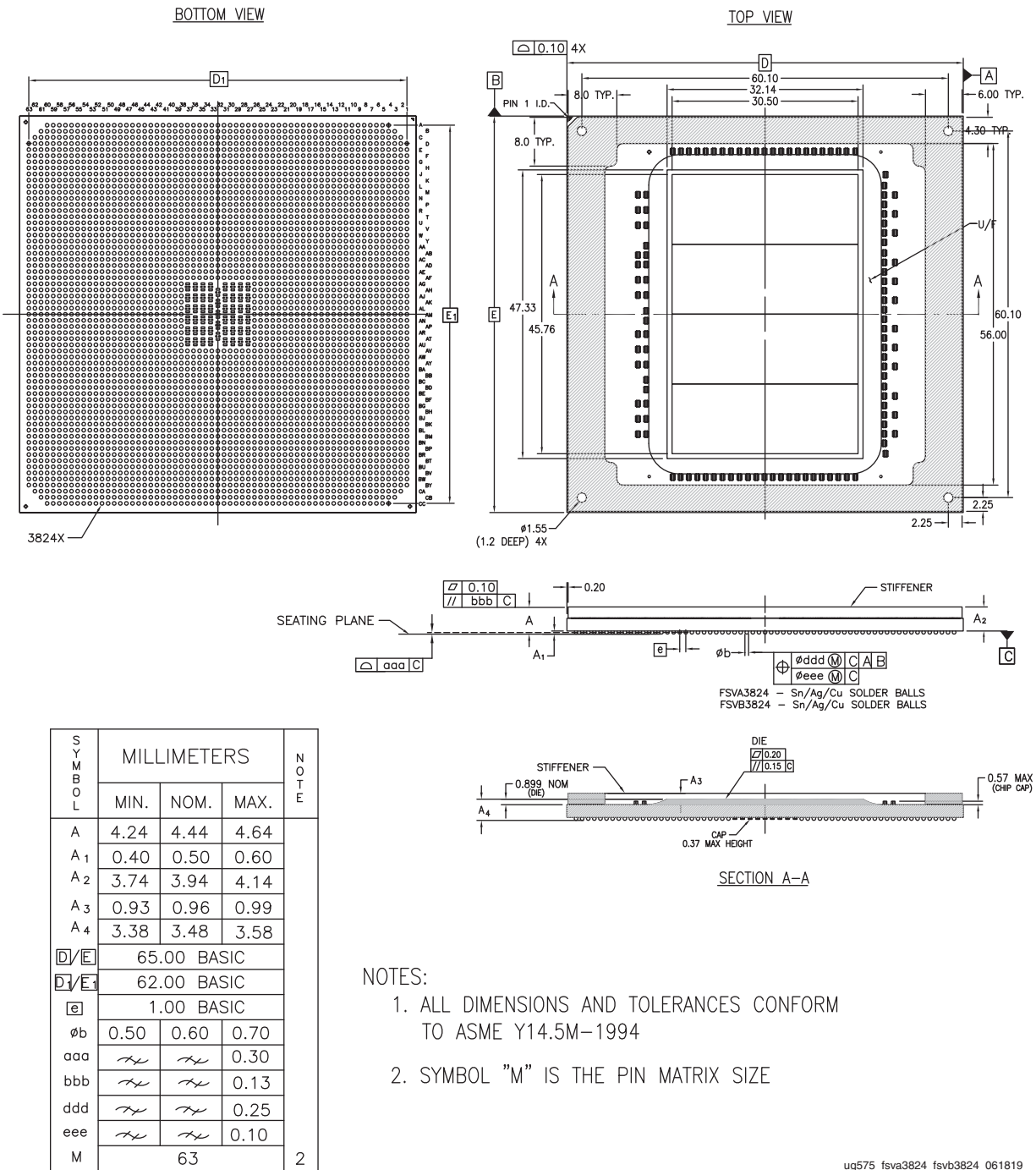
Figure 4-58: Package Dimensions for FSVA3824 and FSVB3824 (XCVU19P)
