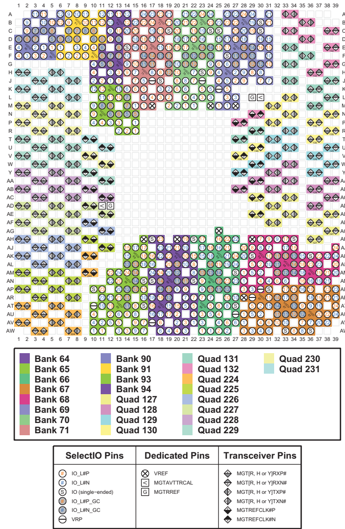
Figure 3-97: FFVE1517 Package—XCKU15P and FFRE1517 Package—XQKU15P I/O Bank Diagram
