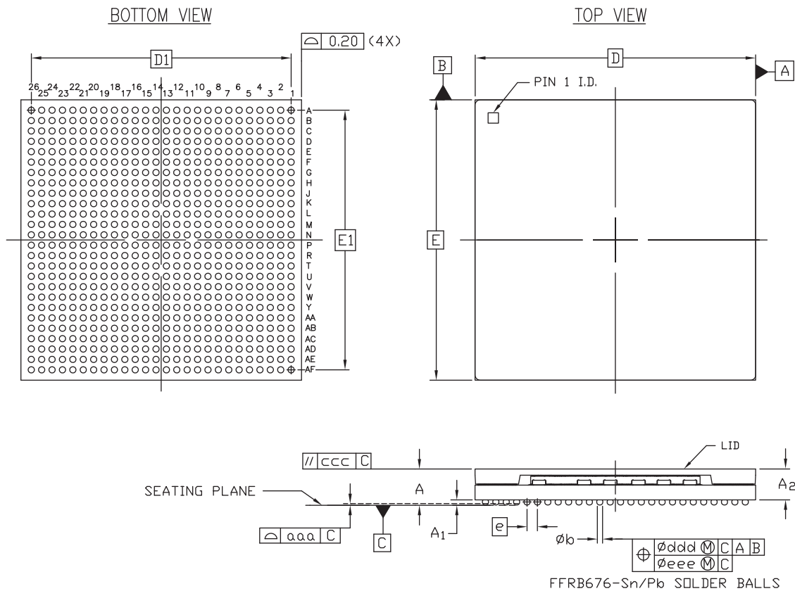
FFRB676-Sn/Pb SOLDER BALLS
