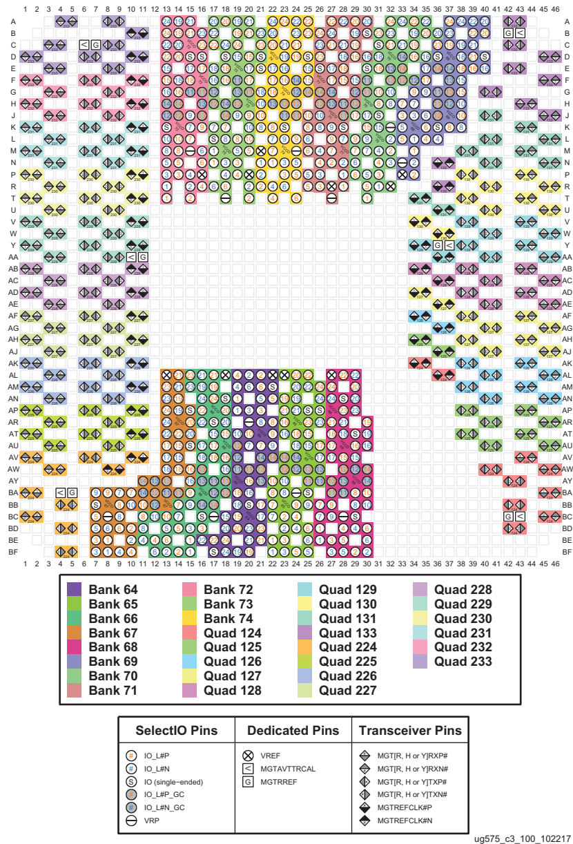
Figure 3-133: FSGD2104 Package—XCVU11P I/O Bank Diagram
