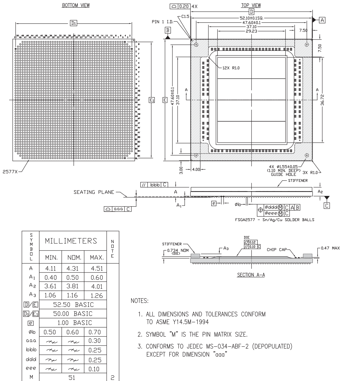
Figure 4-54: Package Dimensions for FSGA2577 (XCVU13P, XCVU27P, and XCVU29P)
