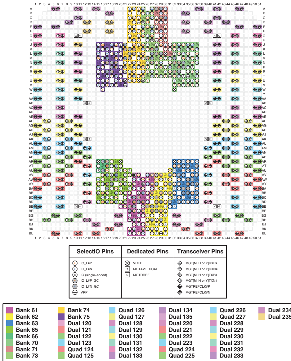
Figure 3-153: FSGA2577 Package—XCVU29P I/O Bank Diagram
