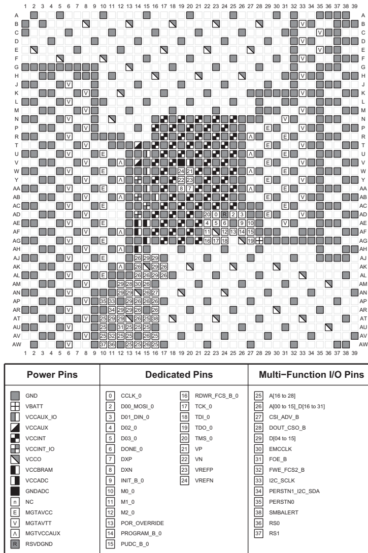
Figure 3-98: FFVE1517 Package—XCKU15P and FFRE1517 Package—XQKU15P Configuration/Power Diagram
