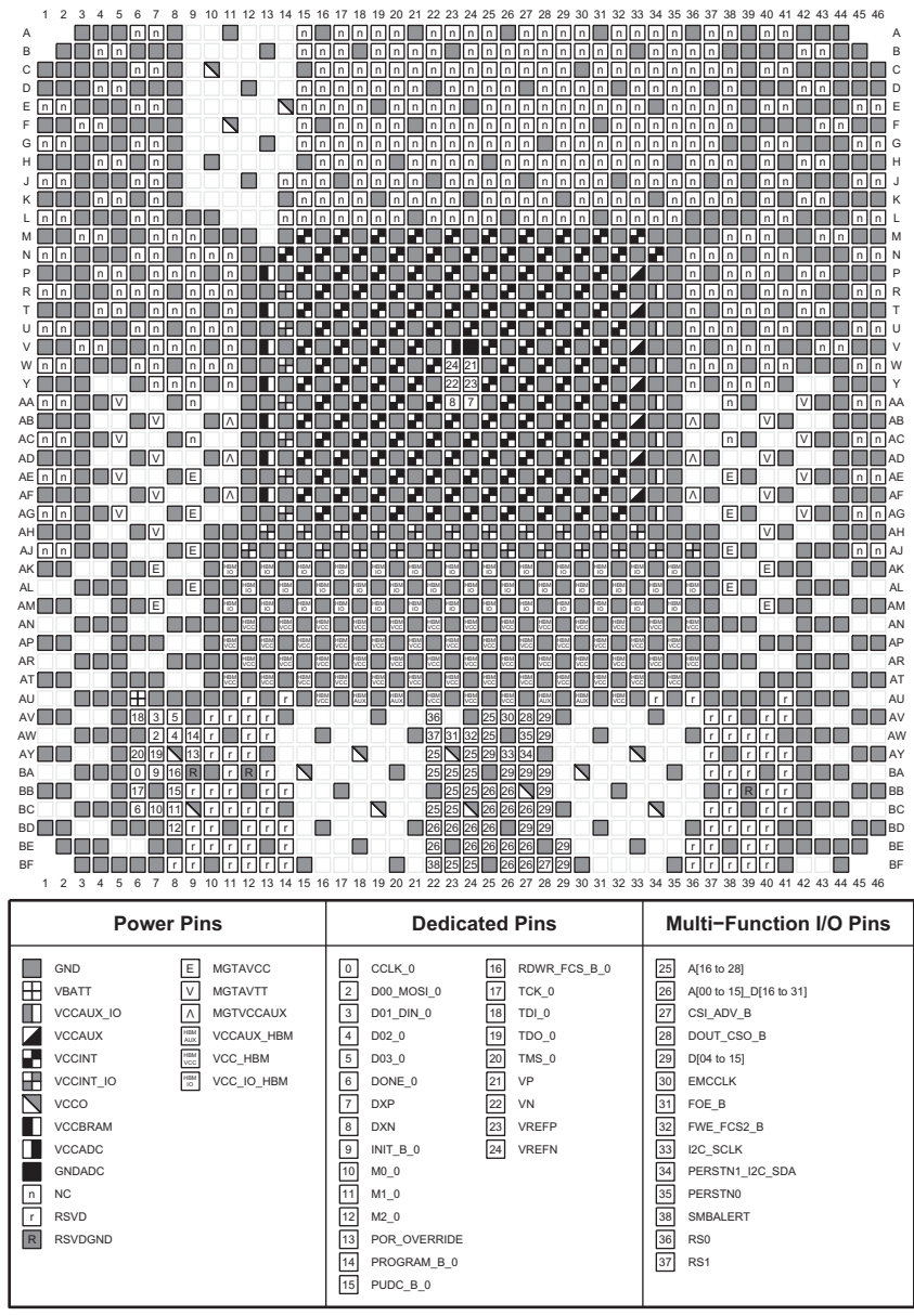
Figure 3-142: FSVH2104 Package—XCVU33P Configuration/Power Diagram
