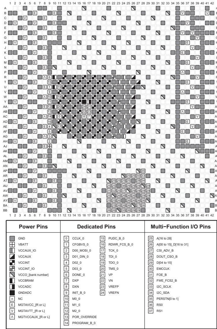
Figure 3-30: FLVB1760 Package—XCKU115 Configuration/Power Diagram
