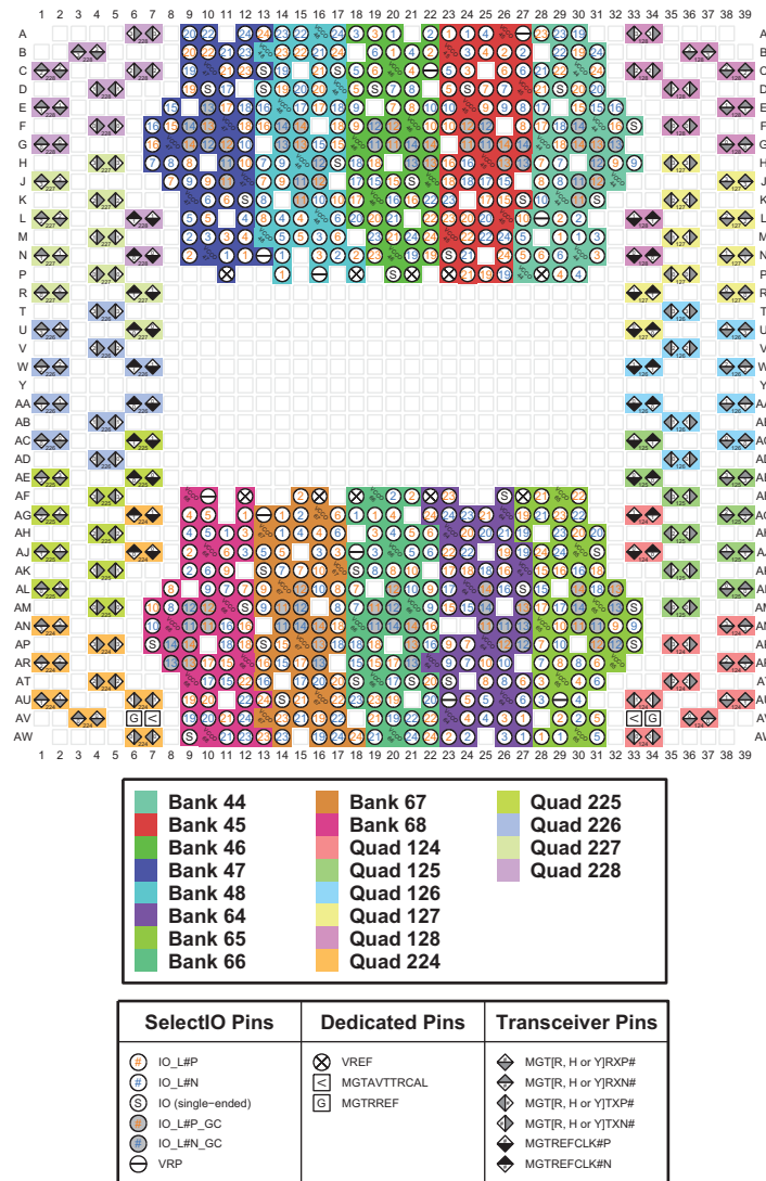
Figure 3-103: FFVC1517 Package—XCVU3P and FFRC1517 Package—XQVU3P I/O Bank Diagram
