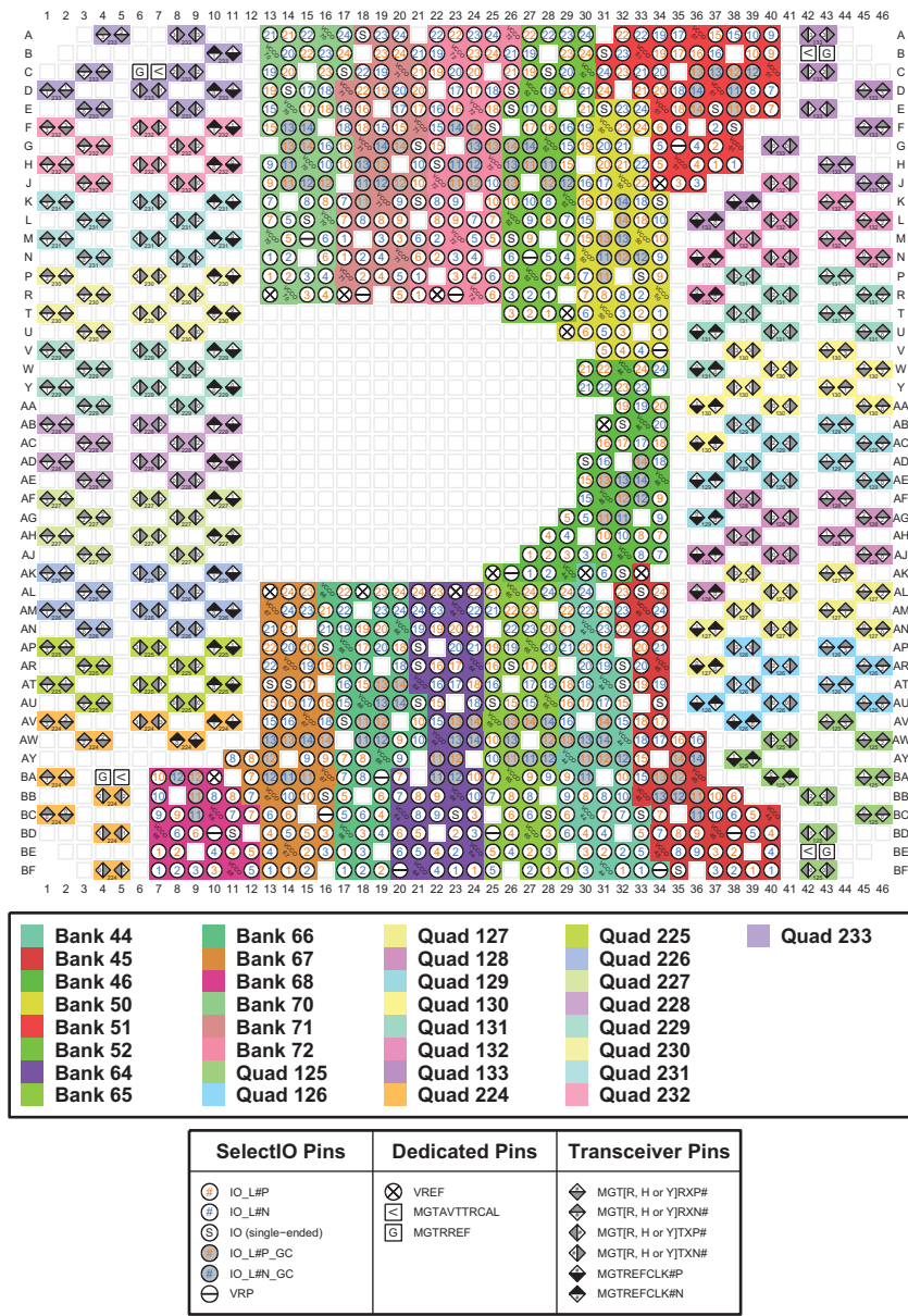
Figure 3-115: FLVB2104 Package—XCVU5P and XCVU7P and FLRB2104 Package—XQVU7P I/O Bank Diagram
