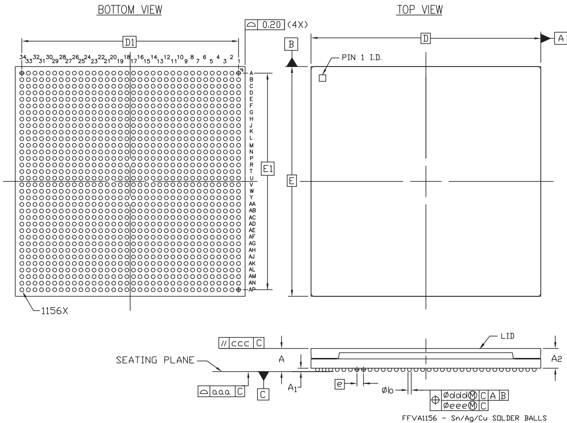
FFVA1156 - Sn/Ag/Cu SOLDER BALLS
