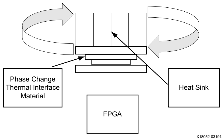
Figure 11-3: Breaking the Bond between Thermal Interface Material and Mated Components
