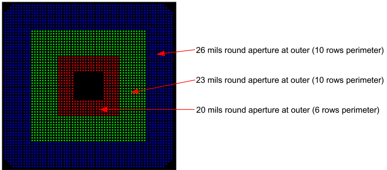
Figure 8-3: Bull's Eye Stencil Aperture
