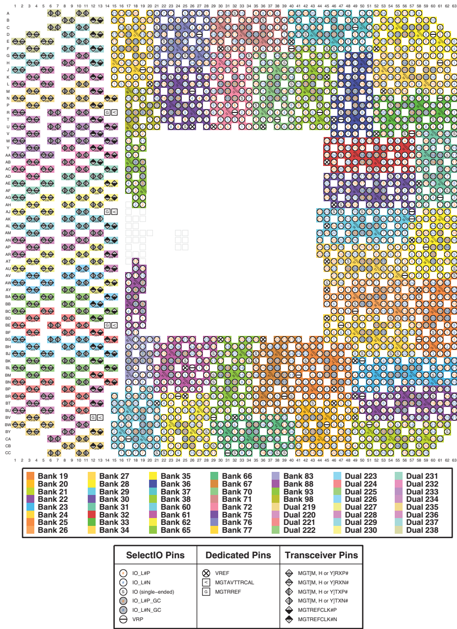
Figure 3-161: FSVB3824 Package—XCVU19P I/O Bank Diagram
