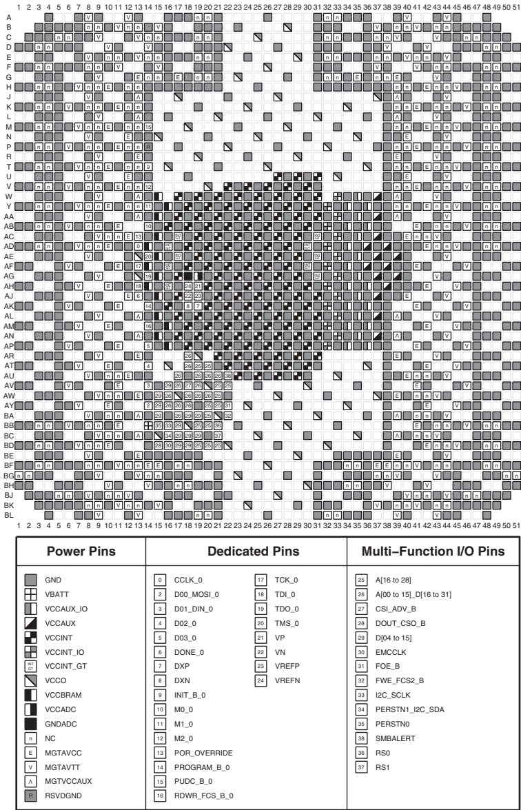
Figure 3-152: FSGA2577 Package—XCVU27P Configuration/Power Diagram
