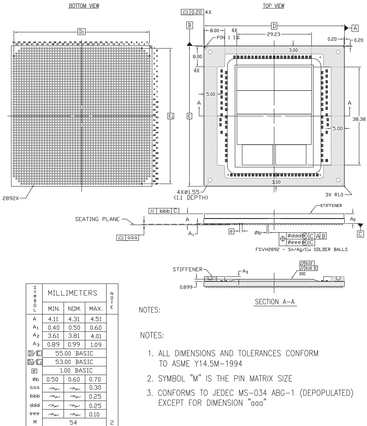
Figure 4-57: Package Dimensions for FSVH2892 (XCVU37P and XCVU47P)
