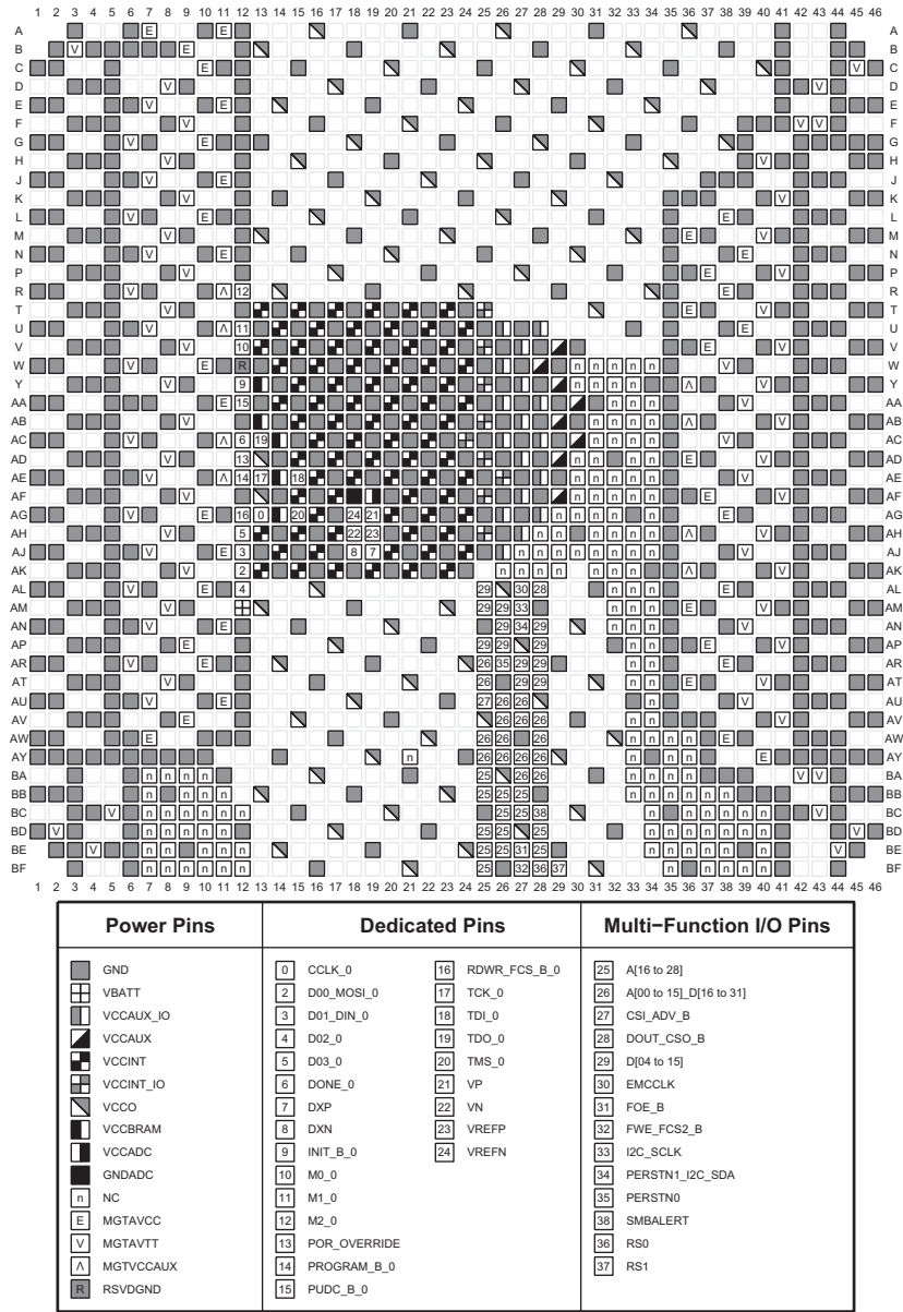
Figure 3-120: FLGB2104 Package—XCVU11P Configuration/Power Diagram
