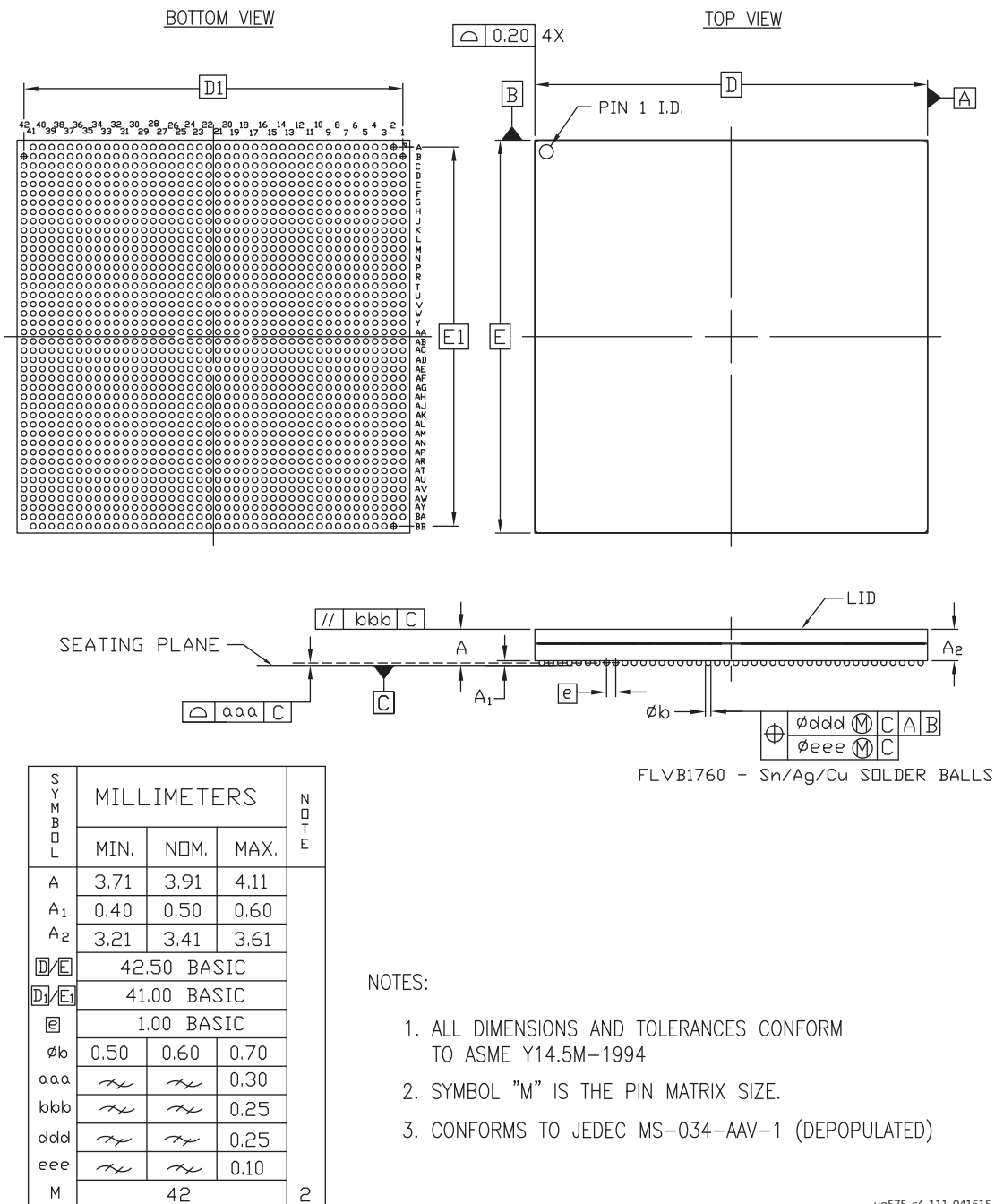
Figure 4-25: Package Dimensions for FLVB1760 (XCKU085, XCKU115, and XCVU125)
