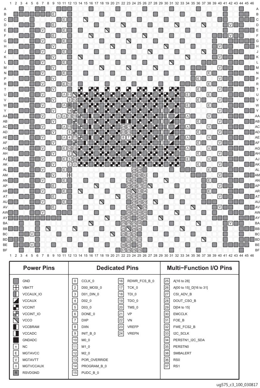
Figure 3-132: FSGD2104 Package—XCVU9P Configuration/Power Diagram
