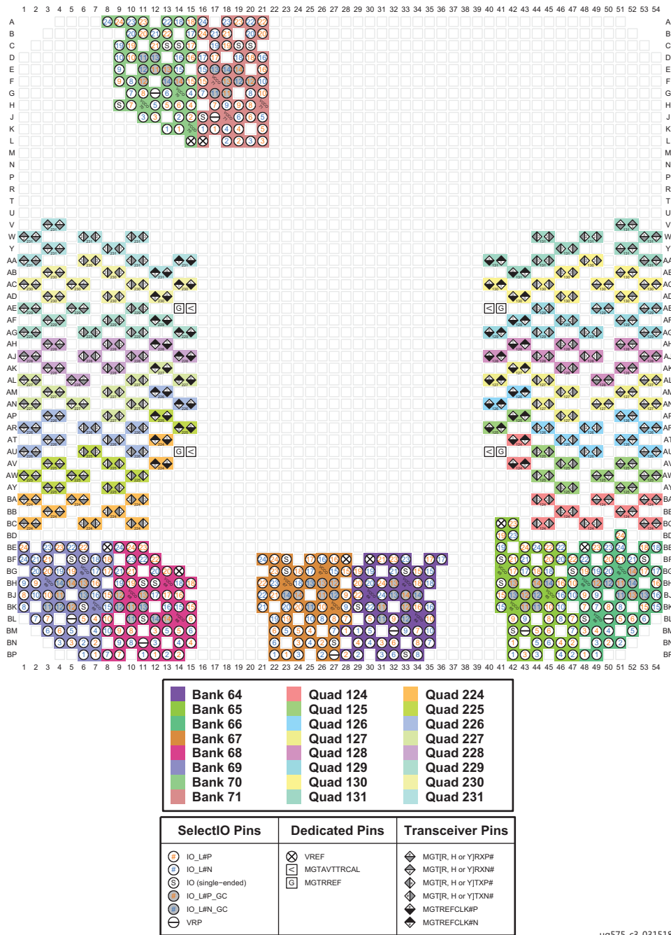
Figure 3-155: FSVH2892 Package—XCVU35P and XCVU45P I/O Bank Diagram
