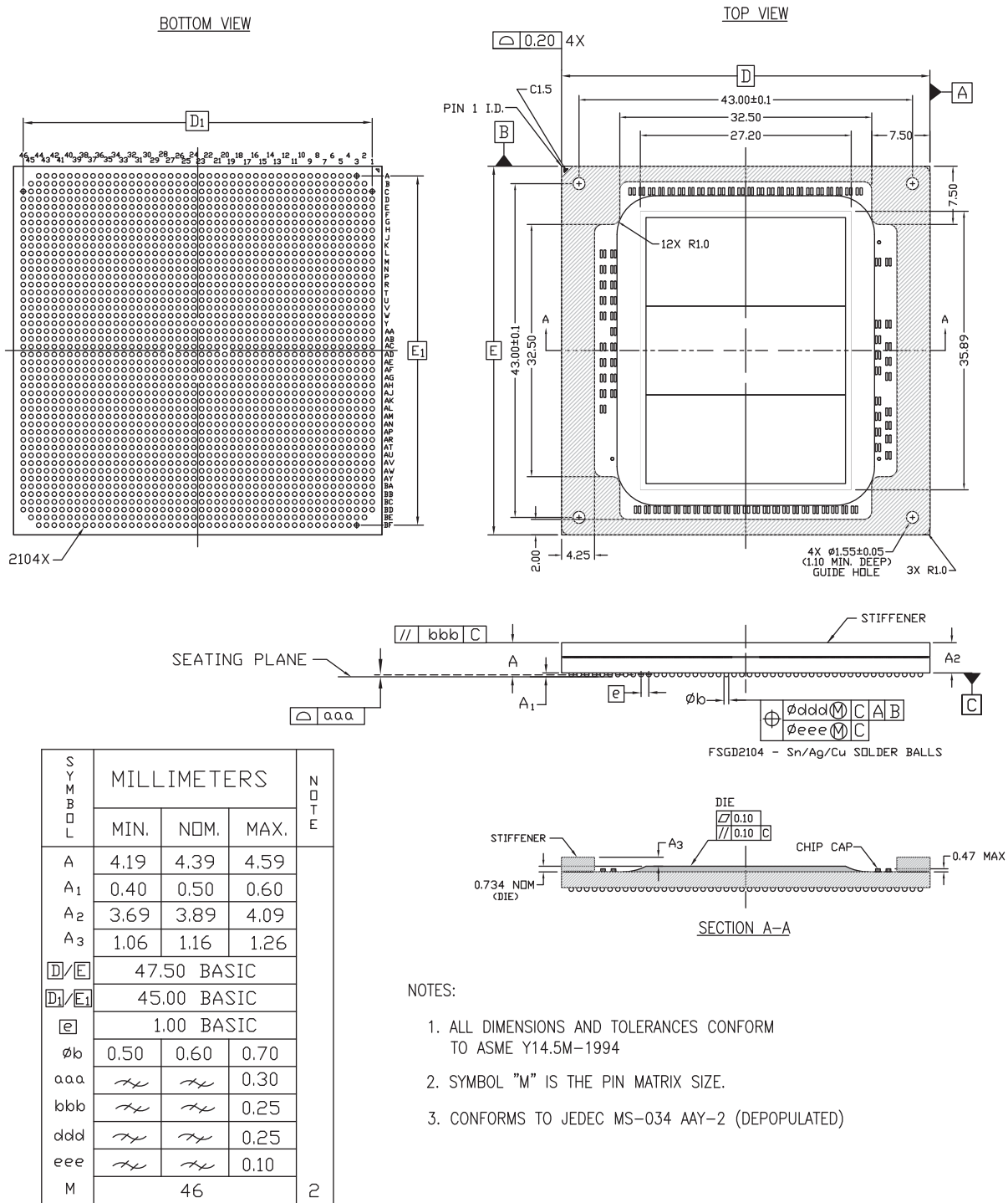
Figure 4-46: Package Dimensions for FSGD2104 (XCVU9P)
