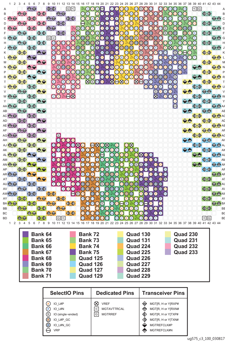
Figure 3-105: FLGF1924 Package—XCVU11P I/O Bank Diagram
