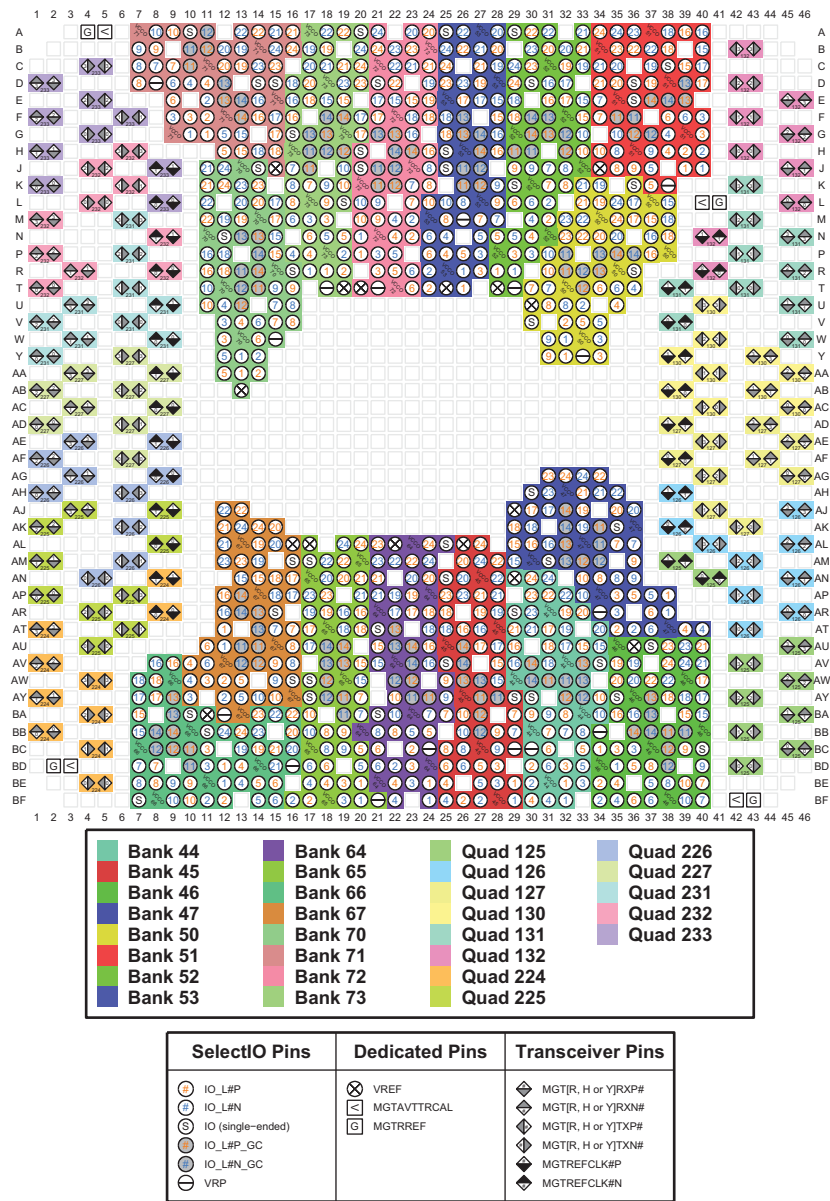
Figure 3-109: FLVA2104 Package—XCVU5P and XCVU7P and FLRA2104 Package—XQVU7P I/O Bank Diagram
