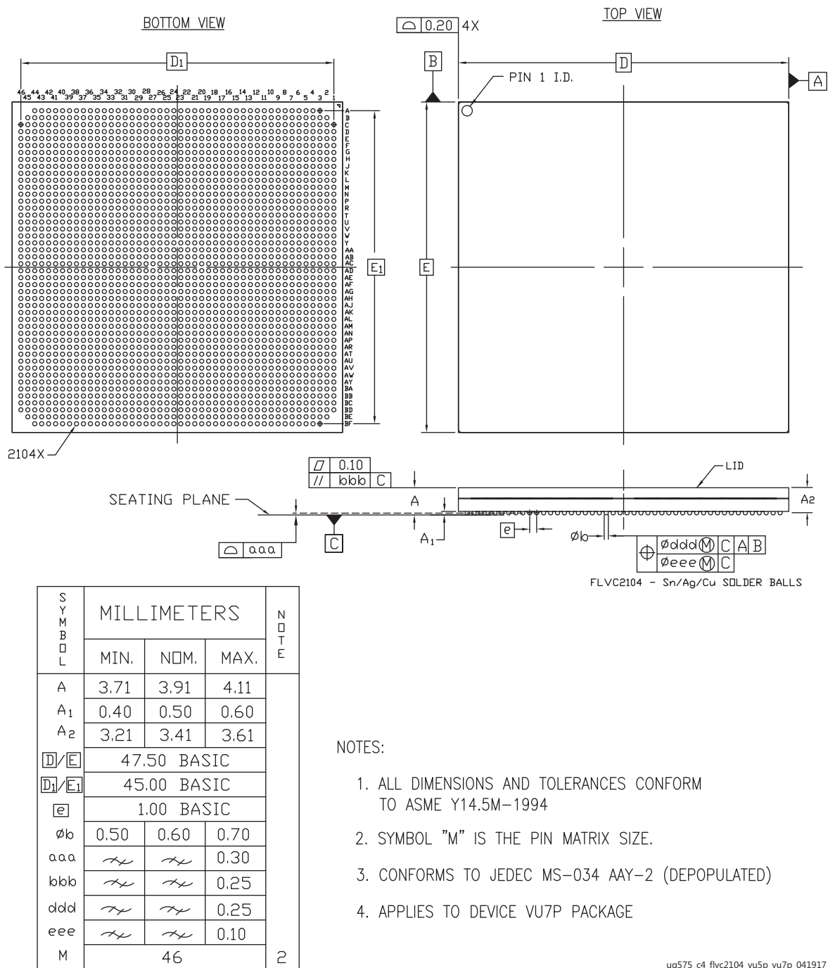
Figure 4-44: Package Dimensions for FLVC2104 (XCVU5P and XCVU7P)
