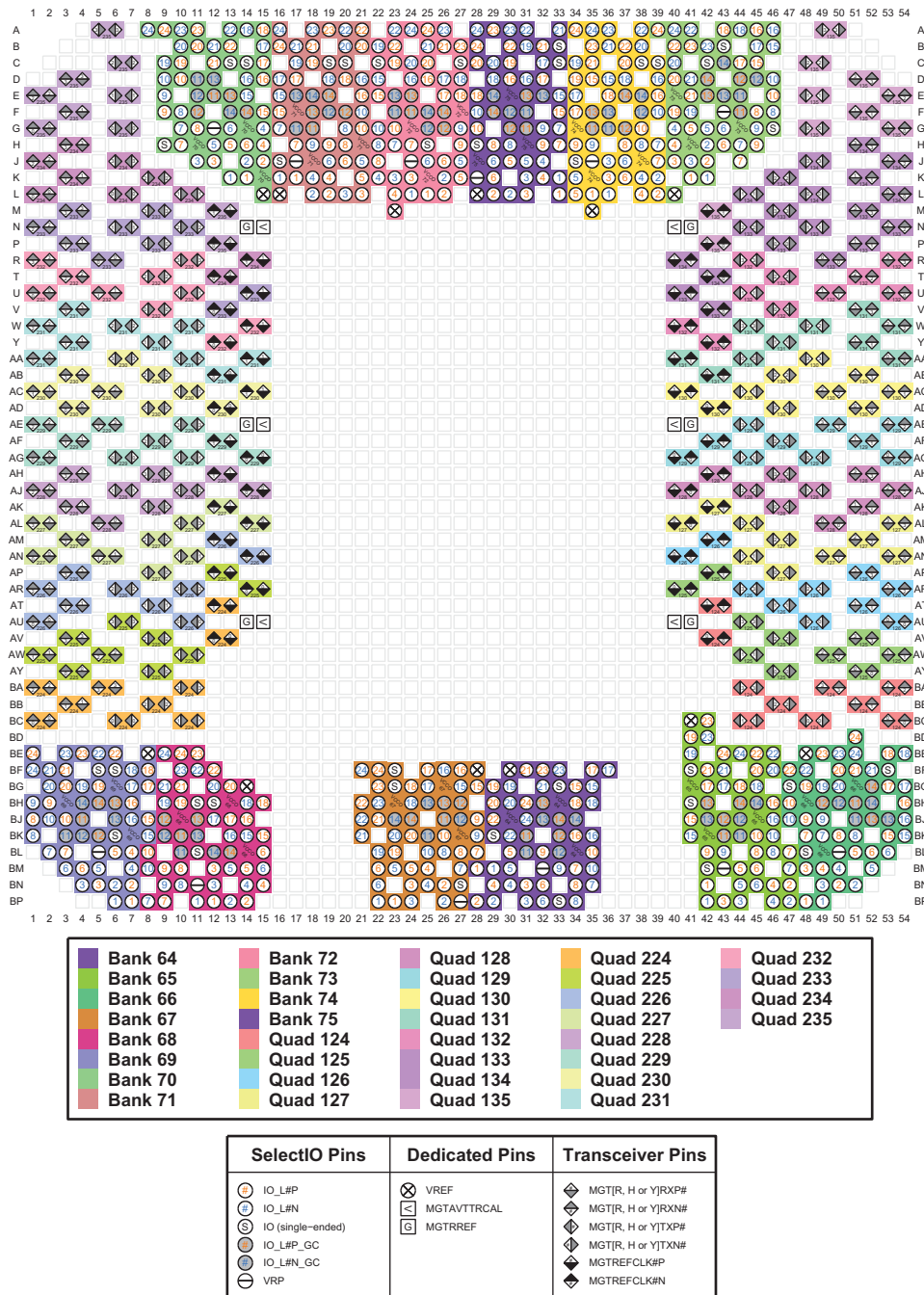
Figure 3-157: FSVH2892 Package—XCVU37P and XCVU47P I/O Bank Diagram
