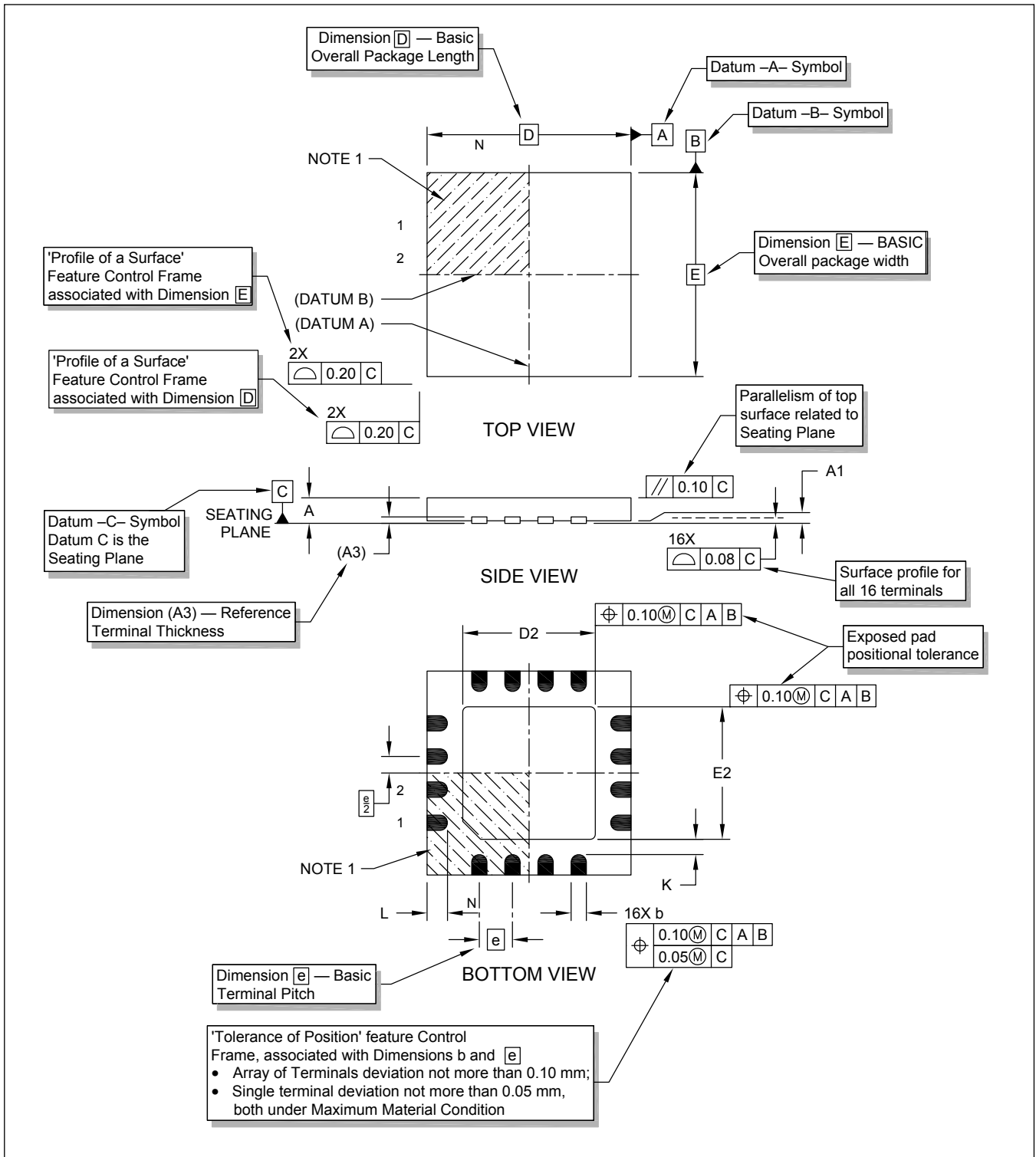
Figure 14. Annotated Package Outline Drawing
