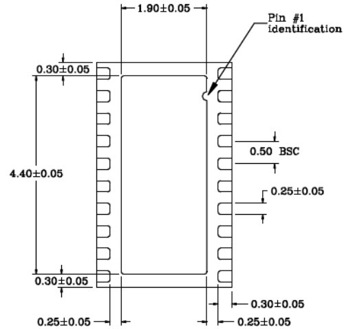
Bottom View NOTE: 2,3
