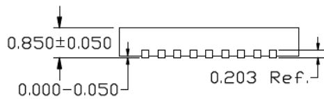
SIDE VIEW NOTE 1, 2, 3
