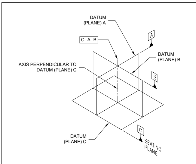
Figure 10. Typical Datums in a Package Outline Drawing
