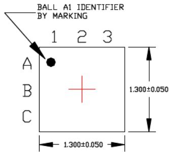
TOP VIEW NOTE: 1,2
