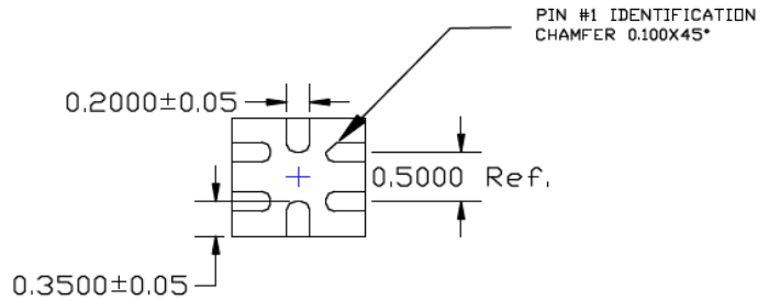
BOTTOM VIEW NOTE: 1, 2, 3
