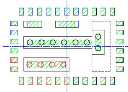
STACKED-UP
