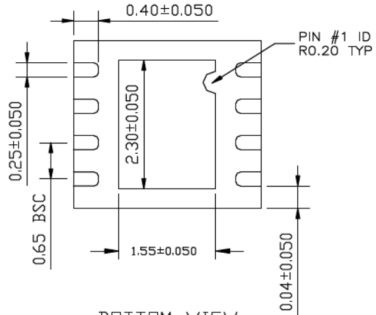
BOTTOM VIEW NOTE: 1, 2, 3
