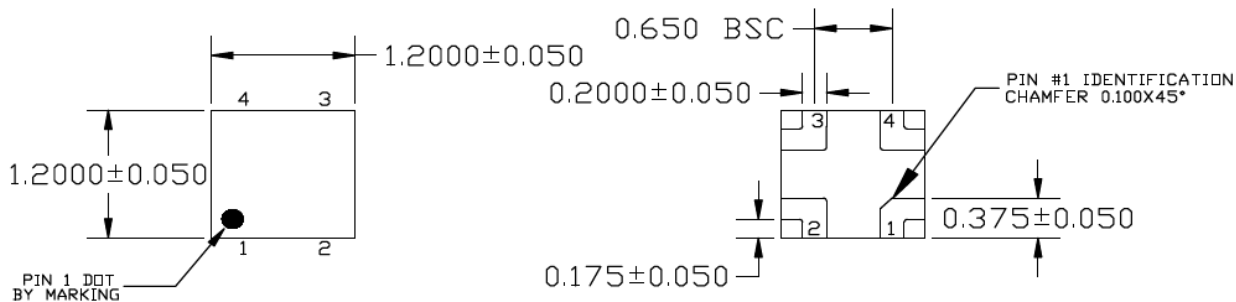
BOTTOM VIEW
