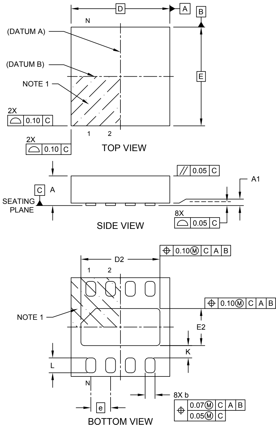
Microchip Technology Drawing C04-200A Sheet 1 of 2
