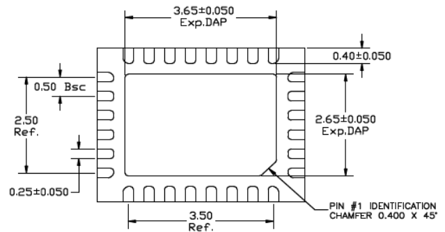
BOTTOM VIEW NOTE: 1, 2, 3
