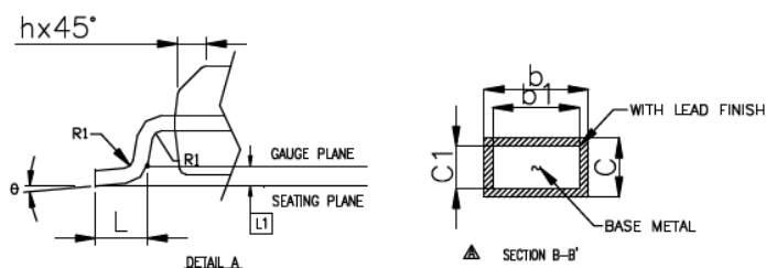
DETAILED VIEW
