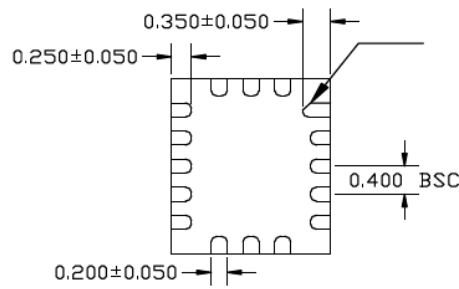
BOTTOM VIEW NOTE: 1, 2, 3
