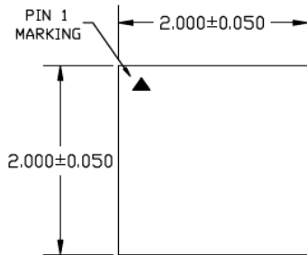
TOP VIEW NOTE: 1,2,3,4
