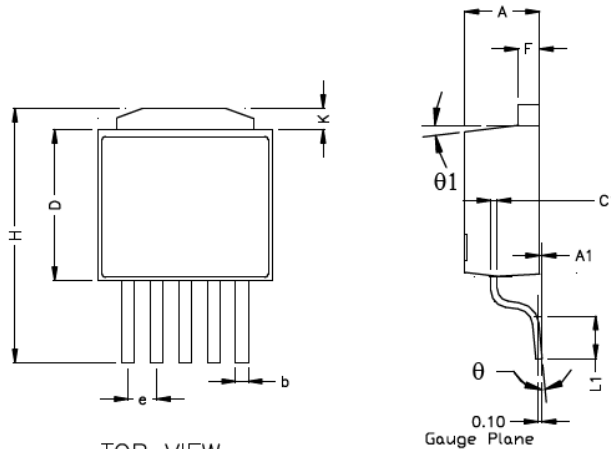
SIDE VIEW 1
