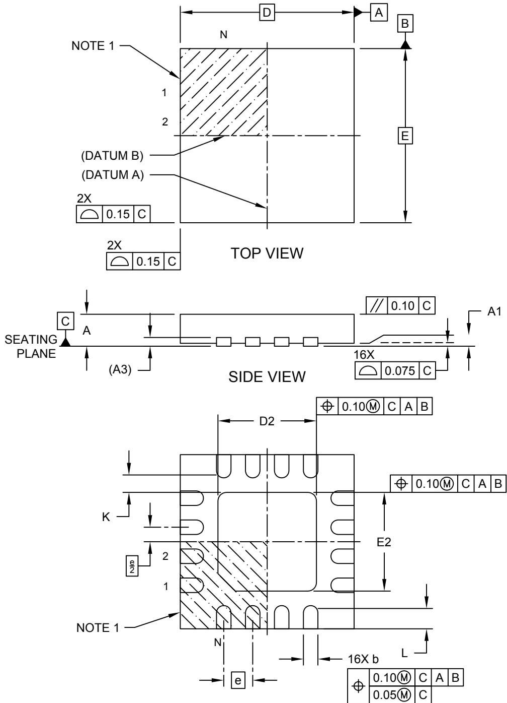
Microchip Technology Drawing C04-253A Sheet 1 of 2
