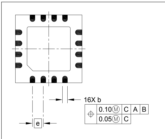
Figure 13. Terminal Pitch, Terminal Width and Tolerance of Position
