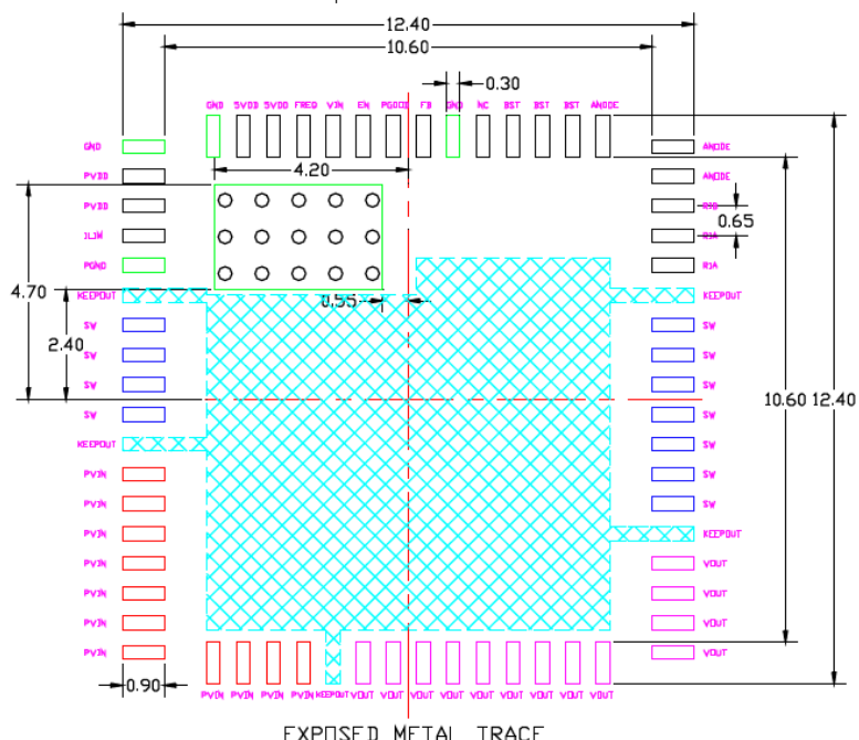
EXPOSED METAL TRACE
