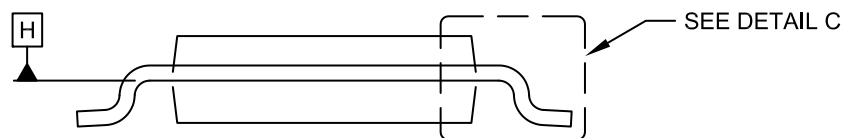
END VIEW
