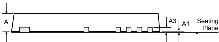
Side View
