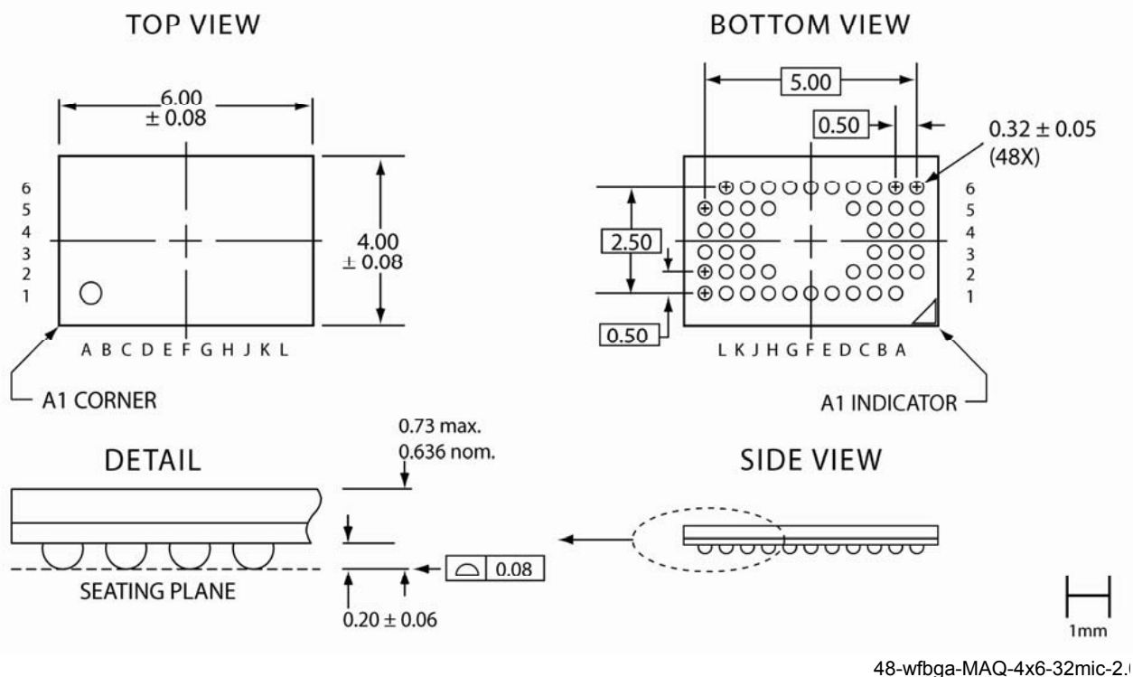
48-wfbga-MAQ-4x6-32mic-2.1
