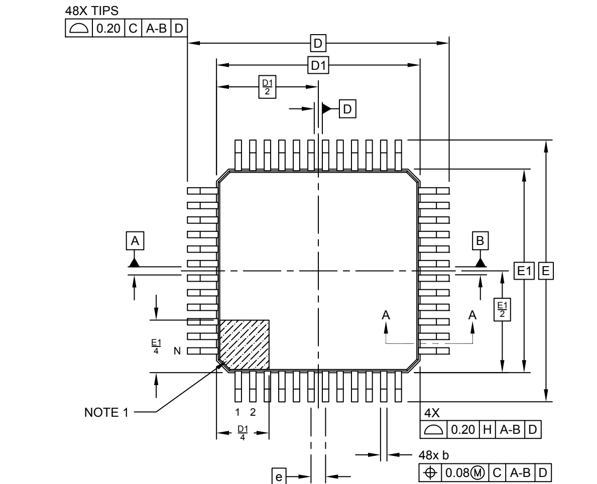
TOP VIEW
