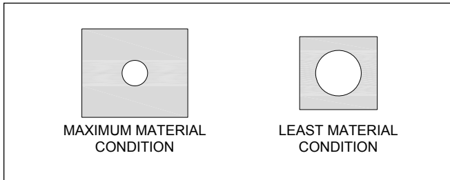
Figure 9. Examples of Maximum Material Condition and Least Material Condition of an object. The shaded areas represent material.
