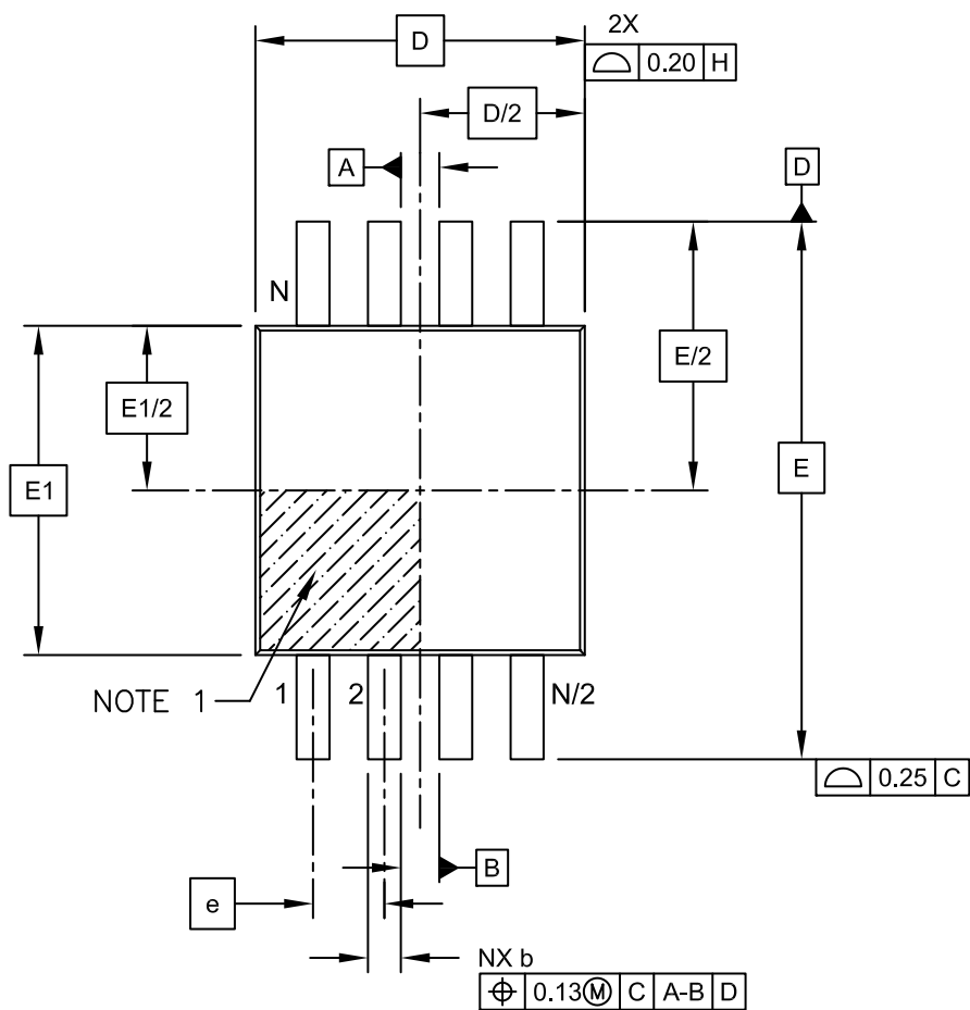
TOP VIEW
