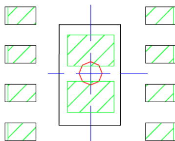
STACKED-UP
