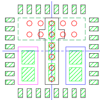
STACKED-UP
