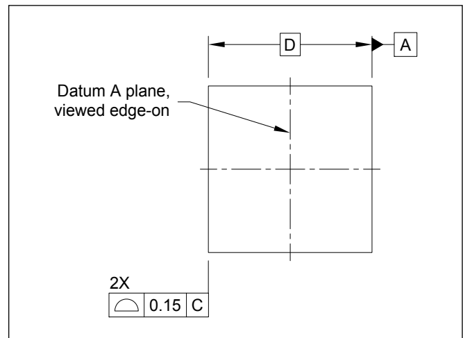
Figure 11. Example of a Datum Plane and Feature Control Frame Related to a Basic Dimension
