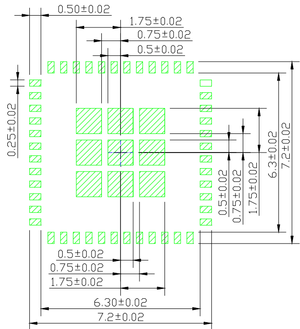
SOLDER STENCIL OPENING
