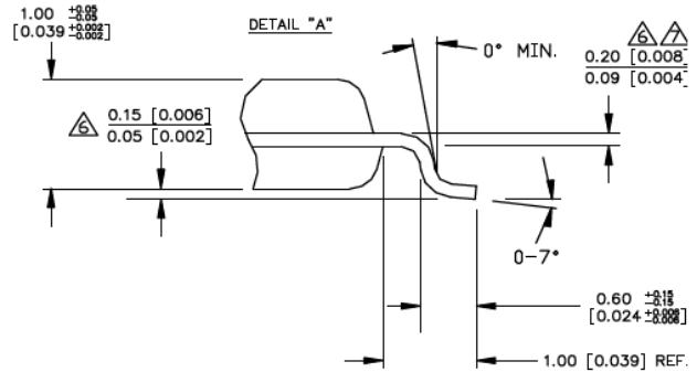
DETAIL VIEW
