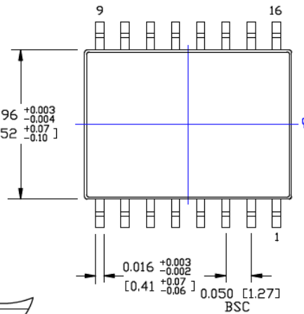
BOTTOM VIEW NOTE 1, 2
