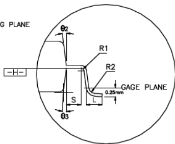
DETAILED VIEW
