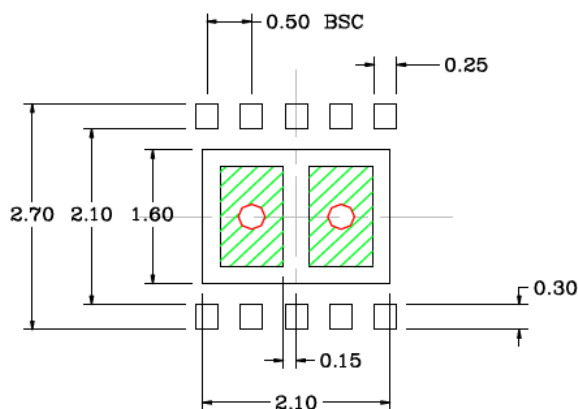
RECOMMENDED LAND PATTERN NOTE: 4, 5, 6
