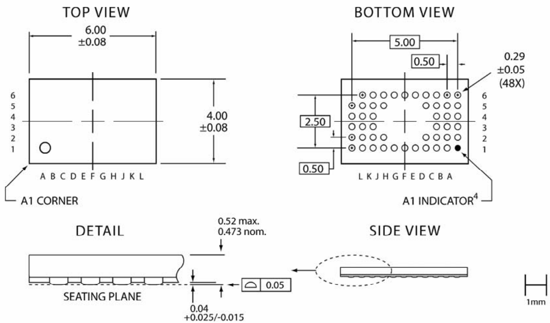
48-xflga-C1Q-4x6-29mic-6.0
