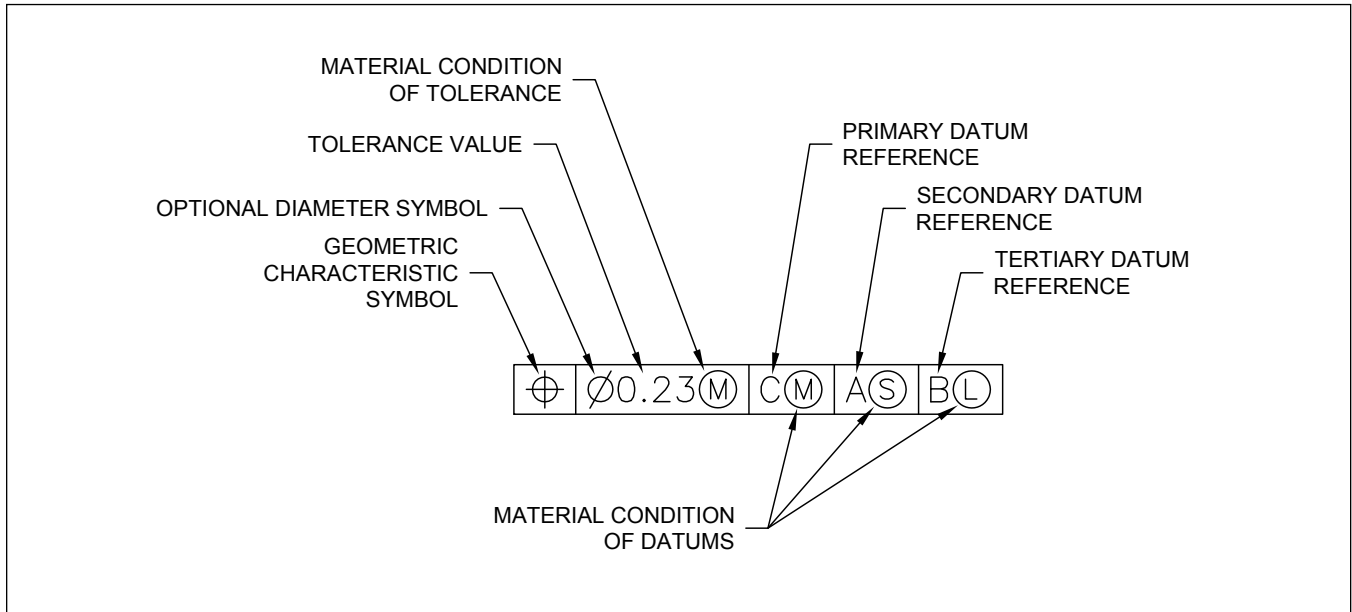
Figure 6. Elements of a Feature Control Frame
