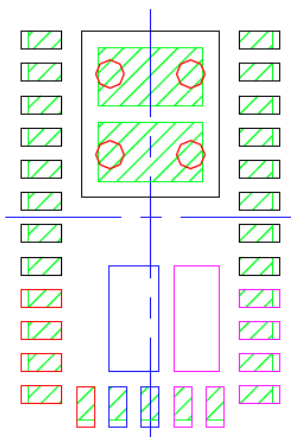
STACKED-UP
