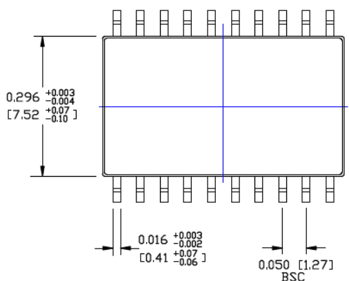
BOTTOM VIEW NOTE 1, 2
