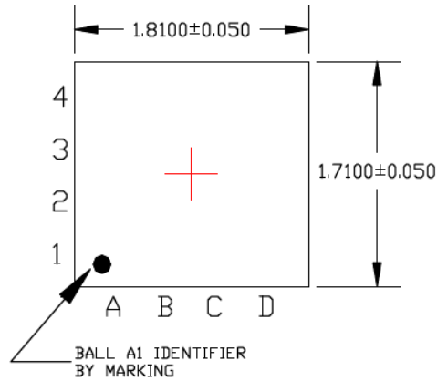
TOP VIEW NOTE: 1, 2
