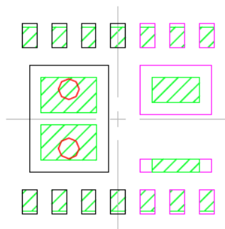
STACKED-UP
