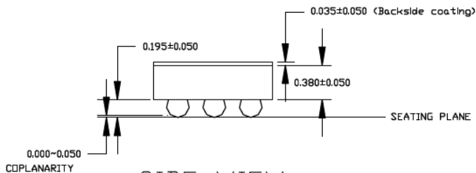
SIDE VIEW NOTE: 1,2
