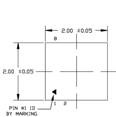
TOP VIEW NOTE: 1, 2, 3
