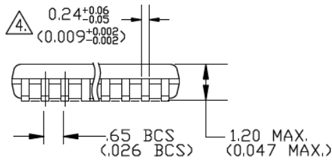
SIDE VIEW NOTES : 1, 2, 4
