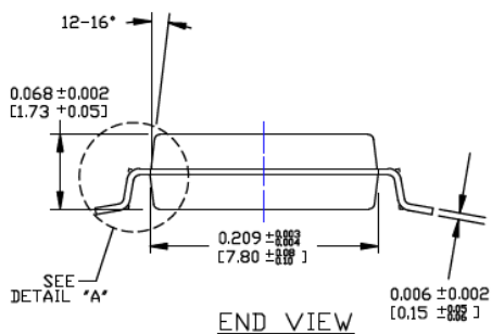
END VIEW NOTE: 1, 2, 3
