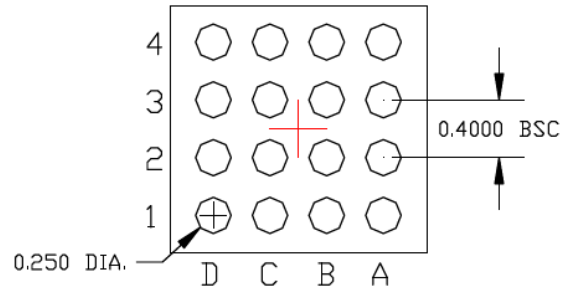
BOTTOM VIEW NOTE: 1, 2
