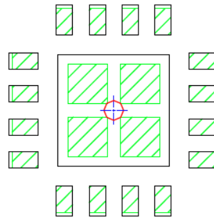
STACKED-UP
