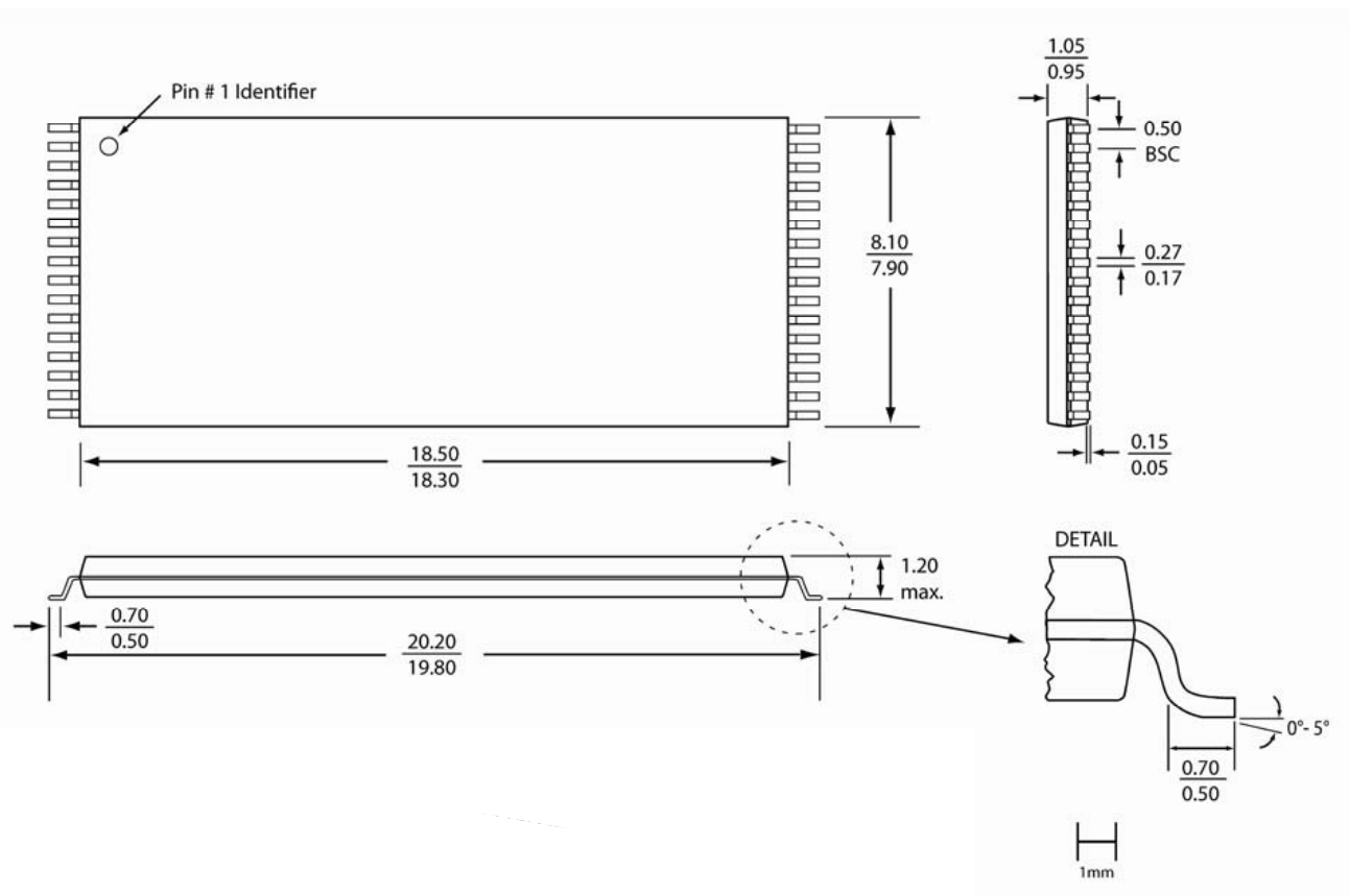
32-tsop-EH-7
