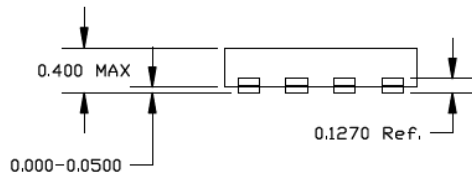
SIDE VIEW NOTE: 1, 2
