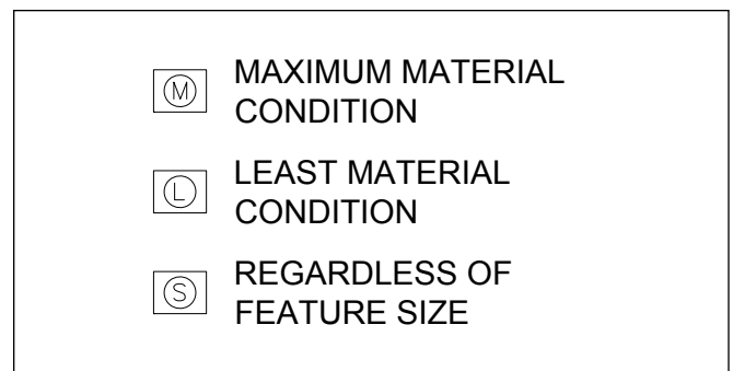
Figure 8. Material Condition Symbols
