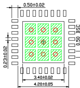
RECOMMENDED LAND PATTERN NOTE: 11, 12
