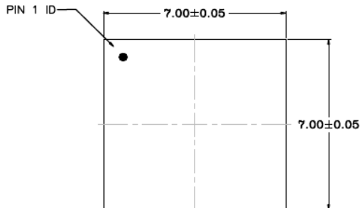
TOP VIEW NOTE: 1, 2, 3, 7
