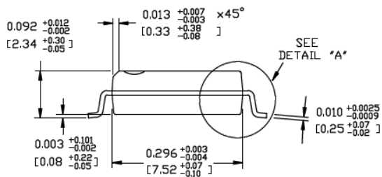
END VIEW NOTE 1, 2, 3
