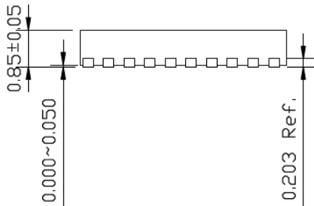
SIDE VIEW NOTE: 1, 2
