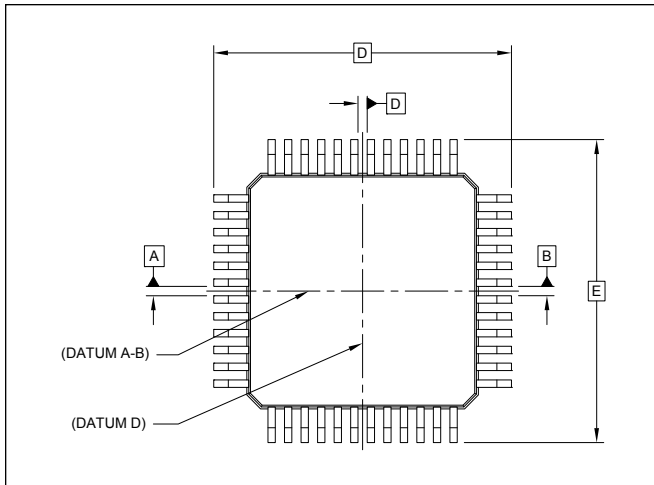
Figure 12. Alternate Datum Definition
