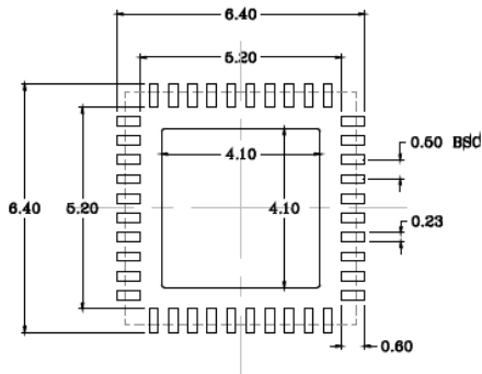
Exposed Metal
