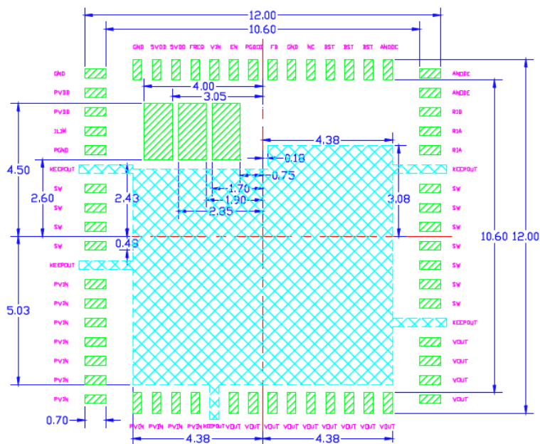
SOLDER STENCIL OPENING
