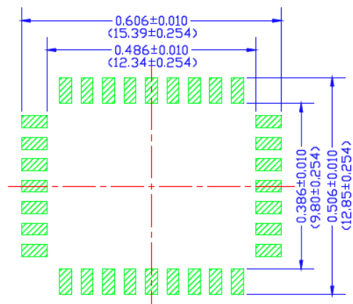
SOLDER STENCIL OPENING
