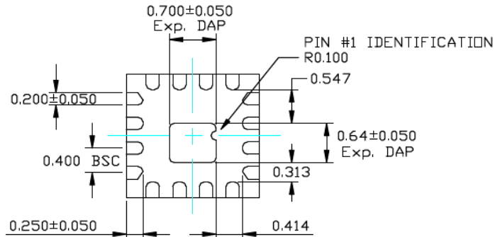
BOTTOM VIEW NOTE: 1, 2, 3, 4
