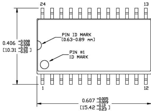
TOP VIEW NOTE 1, 2
