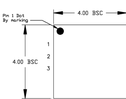
TOP VIEW NOTE: 1, 2, 3
