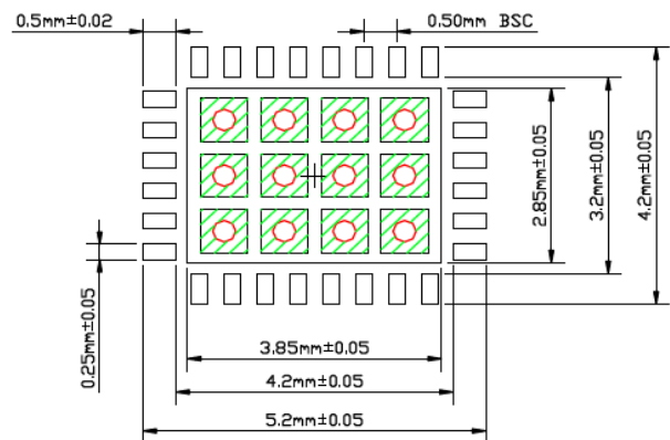
RECOMMENDED LAND PATTERN NOTE: 4, 5
