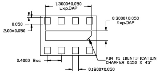
BOTTOM VIEW NOTE: 1, 2, 3
