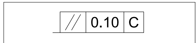
Figure 5. Feature Control Frame
