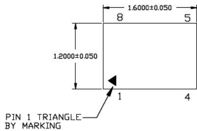
TOP VIEW NOTE: 1, 2
