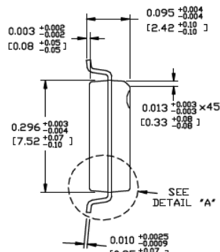
END VIEW
