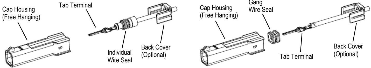
Cap (Free Hanging) Assembly with Gang Wire Seal (1x1 Shown)
