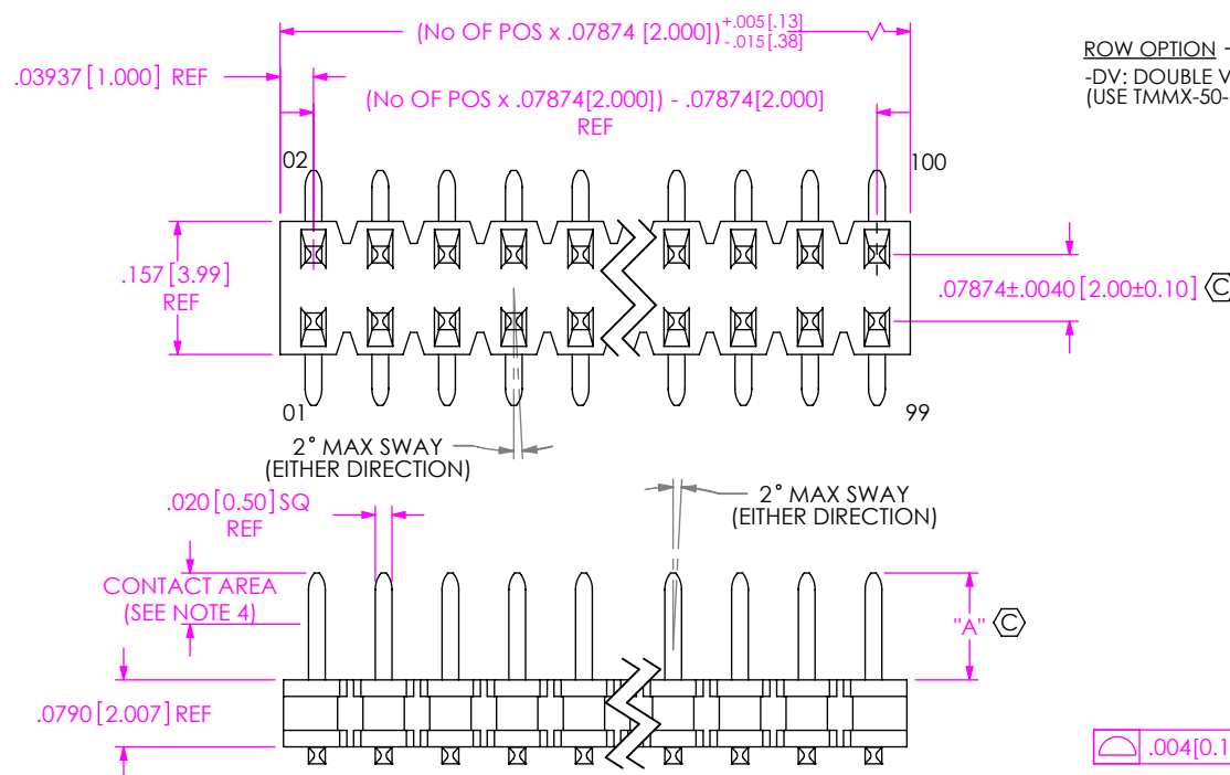
FIG 1 (TMMH-150-XX-XX-DV SHOWN)
