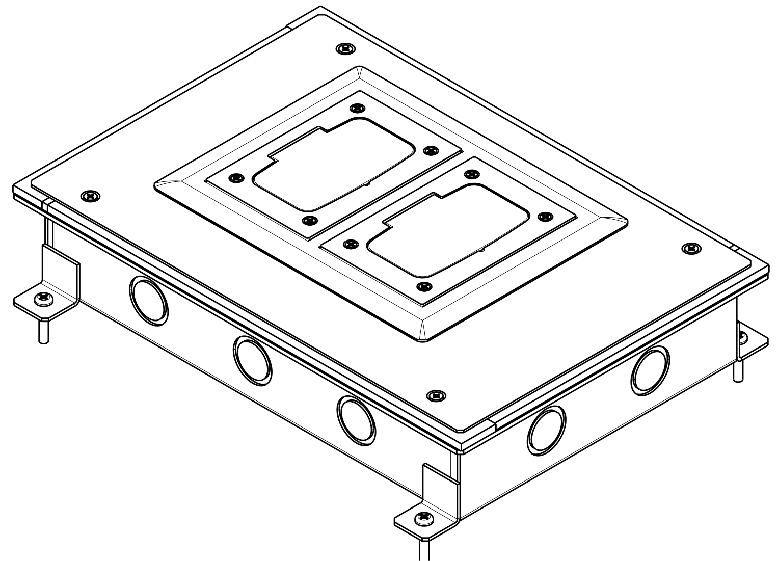
2111353-2 ASSEMBLED
