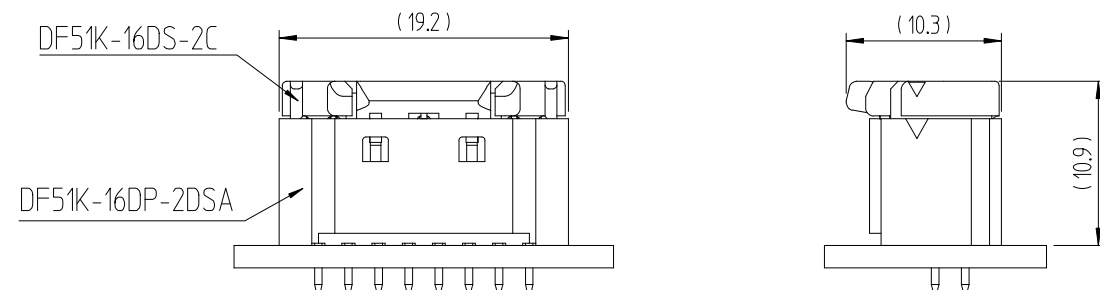
ENGAGEMENT FIGURE (2:1)
