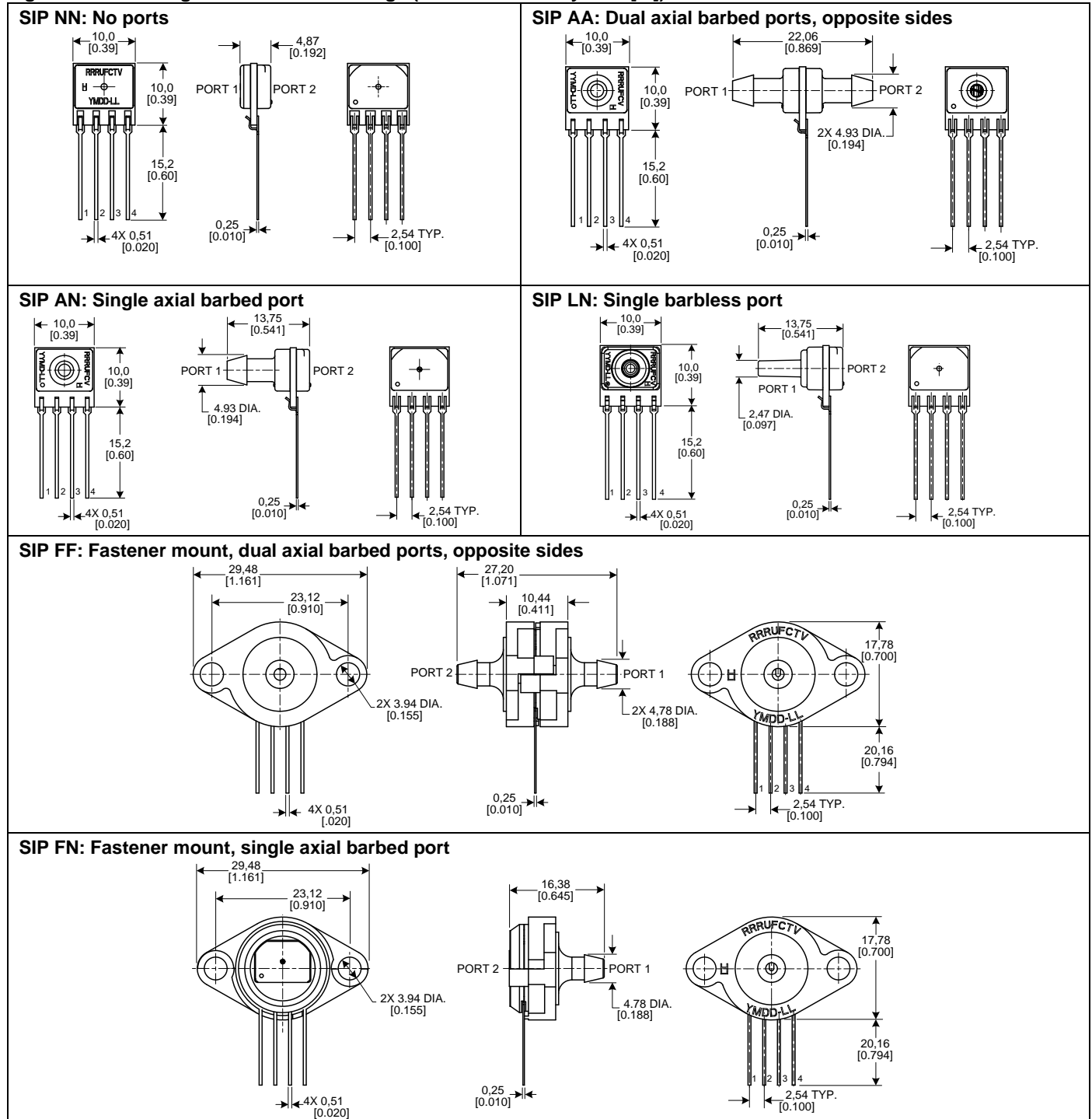
Figure 3. SIP Package Dimensional Drawings (For reference only: mm [in])
