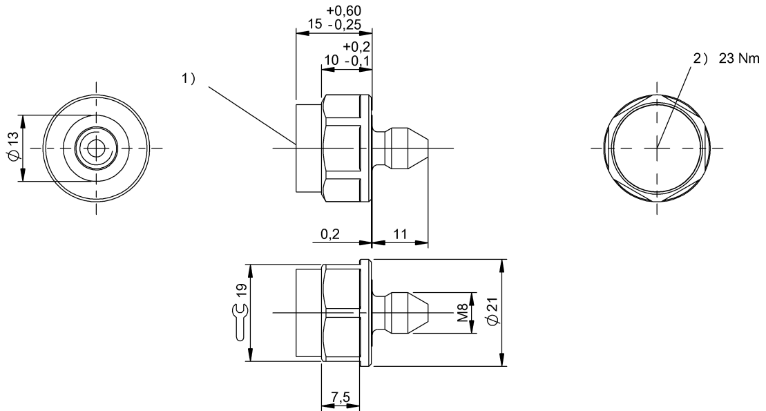
1) Sensing surface, 2) Tightening torque
