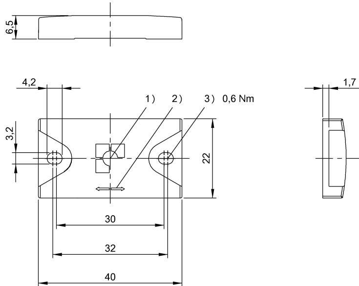
1) Sensing surface, 2) Read/write axis, 3) Tightening torque
