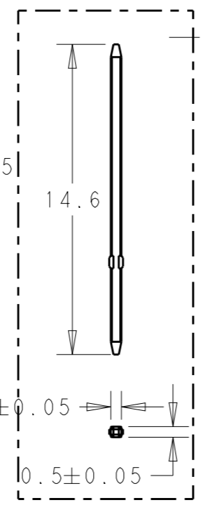
6 Pin
