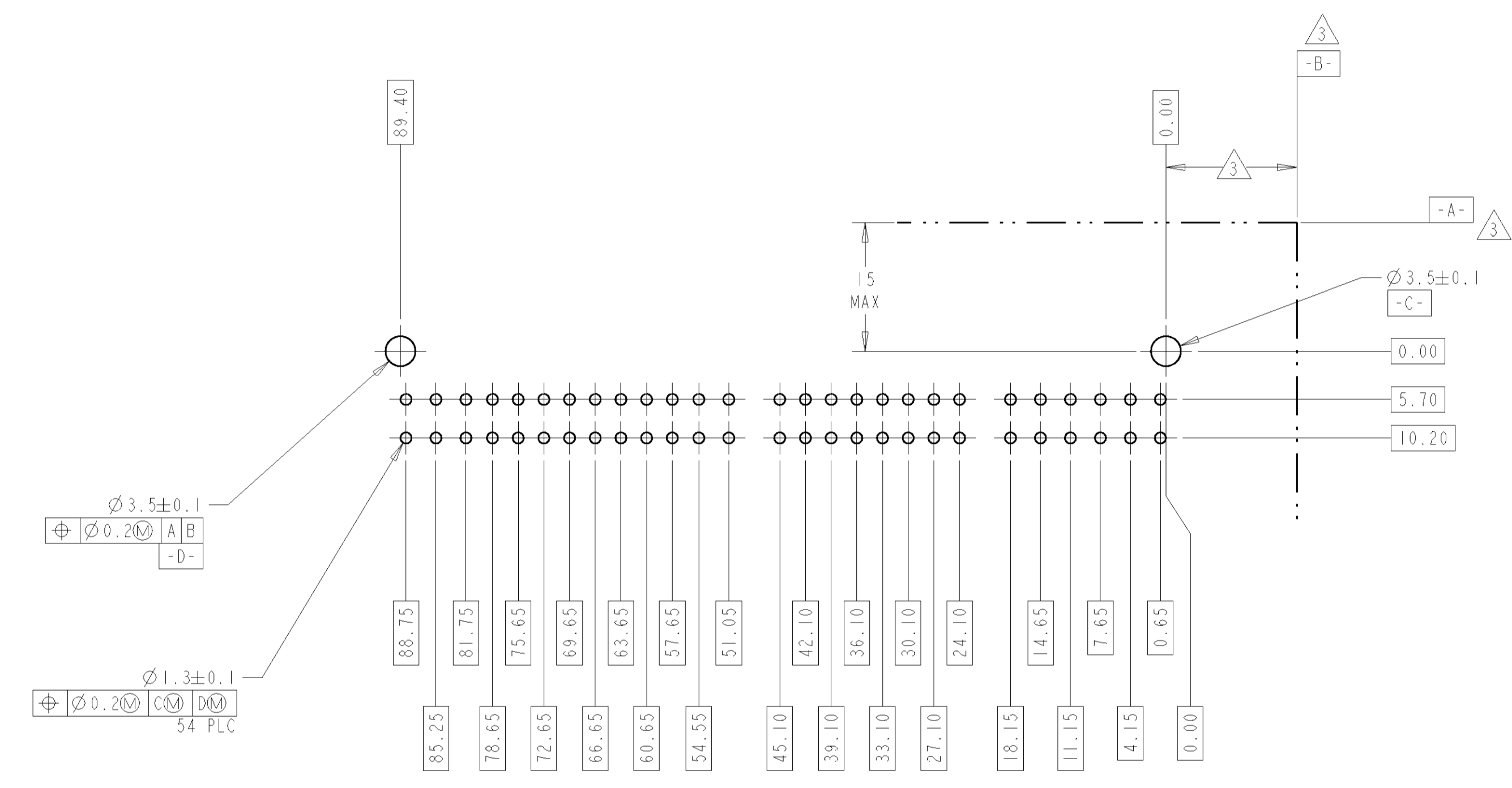
P.C. BOARD LAYOUT
