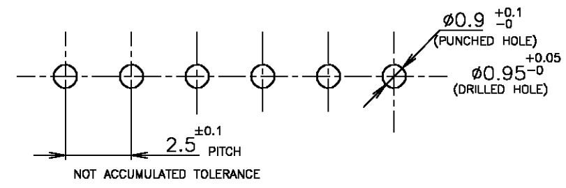
RECOMMENDABLE P.C.BOARD LAYOUT (B.C.B THK:1.0~1.6)
