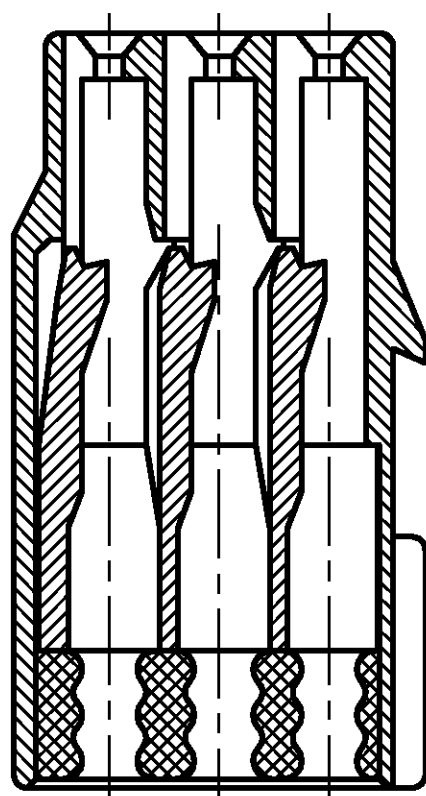
SECT. A-A
