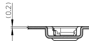
SECTION X-X
