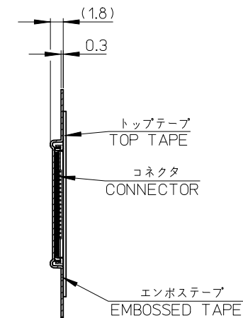
SECTION Y-Y
