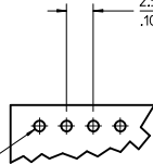
TYP. HOLE PATTERN FOR 1.57/.062 THK. PCB
