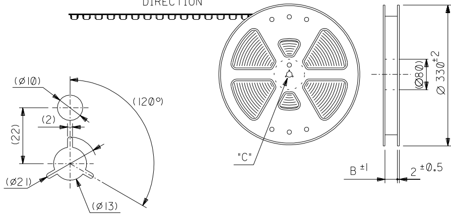
DETAIL "C"
