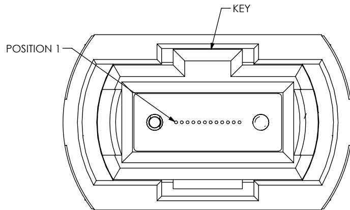
12 FIBER CONNECTOR
