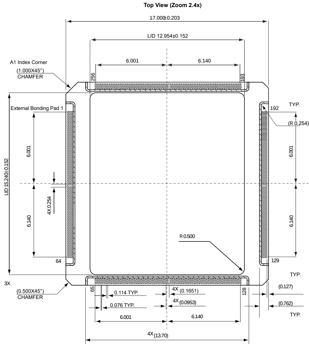
Figure 17 • CCLG Substrate Dimensions
