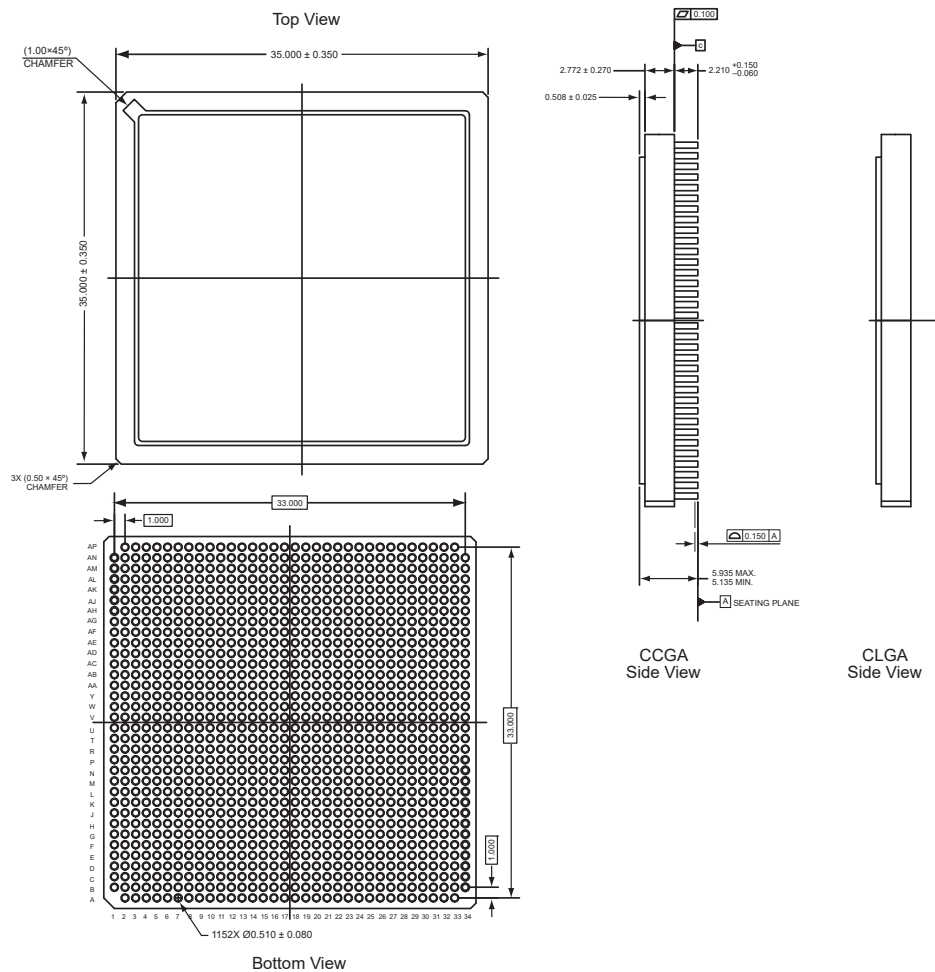
Figure 22 • Package Outline of CG1152
