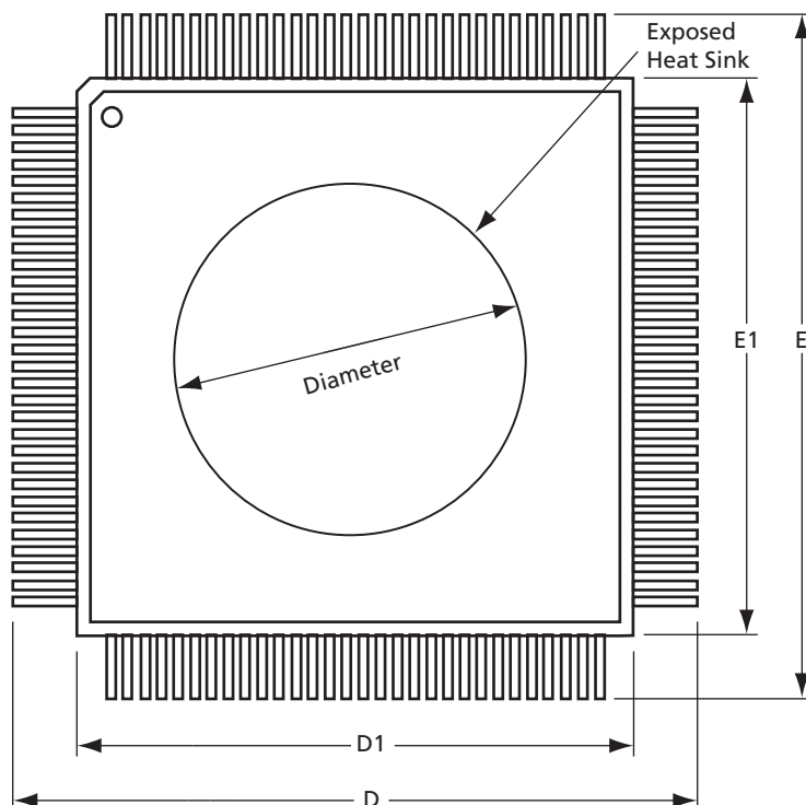
Figure 35 • Plastic Quad Flat Pack—Exposed Heatsink (RQFP)
