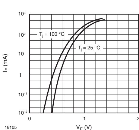
Fig. 1 - Forward Characteristics
