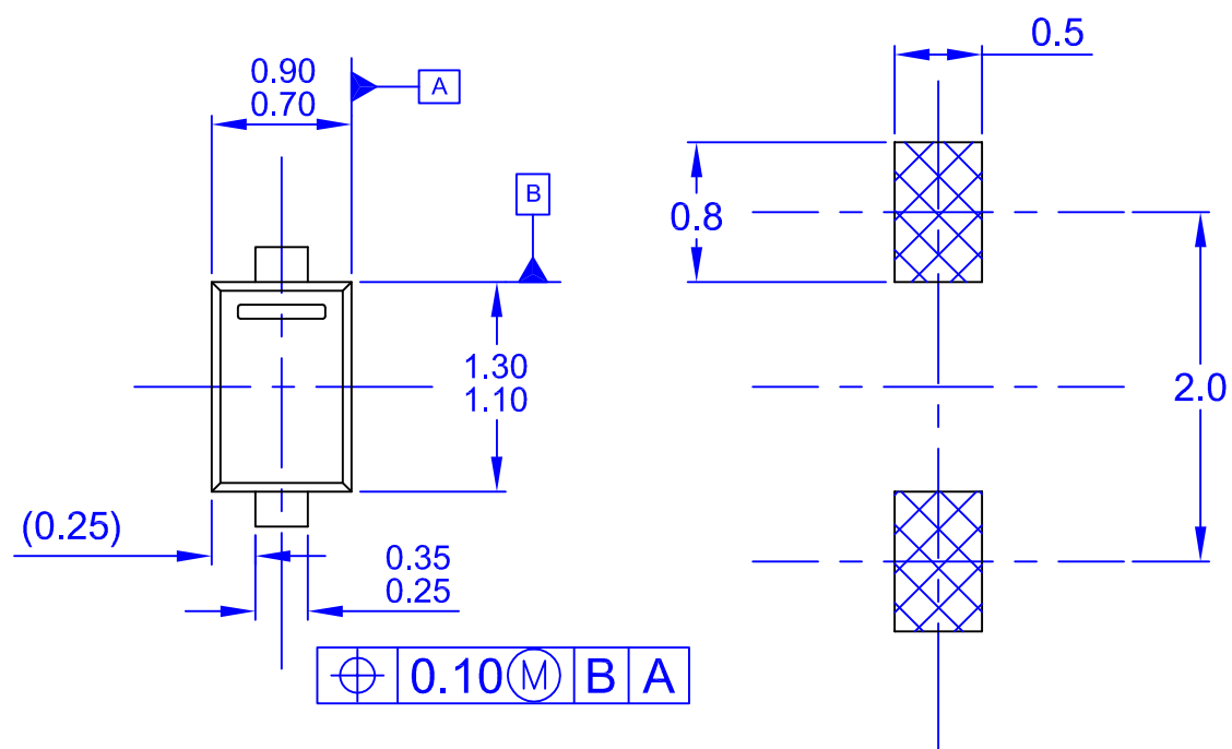
LAND PATTERN RECOMMENDATION
