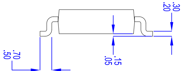
END VIEW
