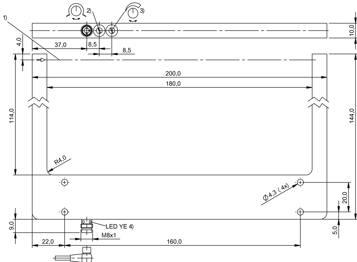
1) Optical axis, 2) Sensitivity, 3) Light-on/dark-on, 4) Output function
