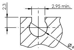
C-Nut z.B. SMC C-slot e.g. SMC
