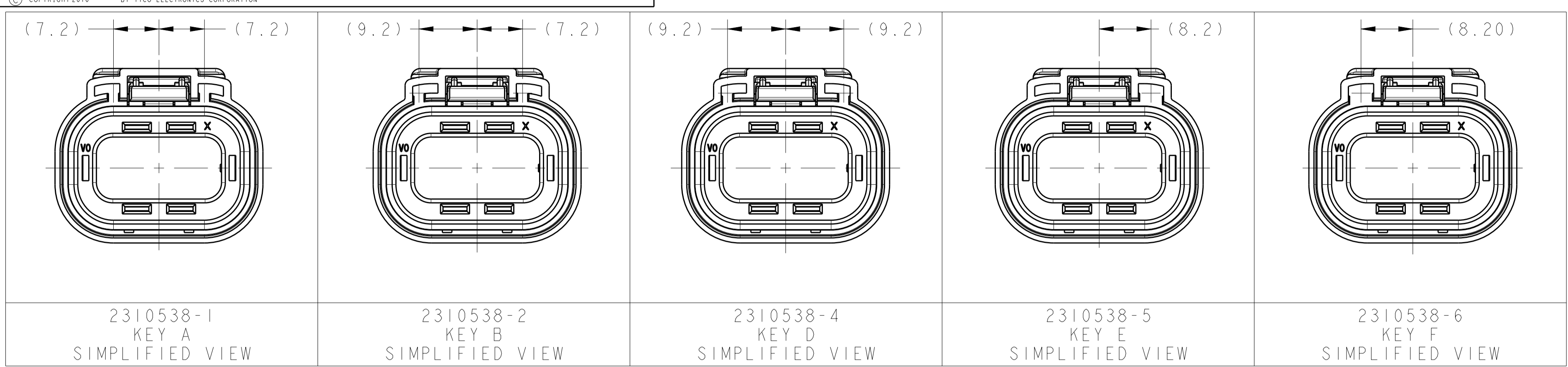
2310538-1 KEY A SIMPLIFIED VIEW 2310538-2 KEY B SIMPLIFIED VIEW 2310538-4 KEY D SIMPLIFIED VIEW 2310538-5 KEY E SIMPLIFIED VIEW 2310538-6 KEY F SIMPLIFIED VIEW
