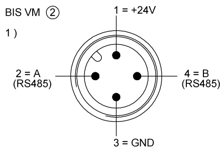
1) View towards connector
