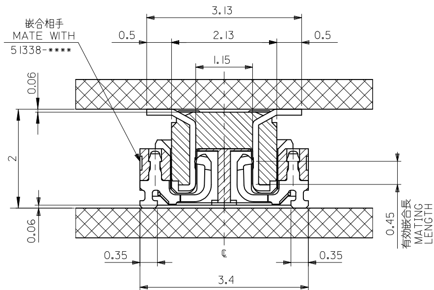
MATED DRAWING (REFERENCE)
