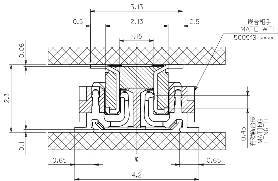
MATED DRAWING (REFERENCE)
