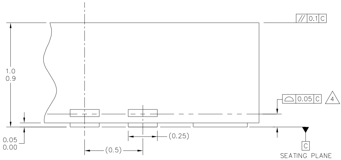
DETAIL G
