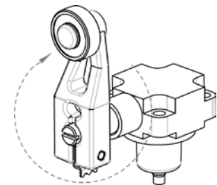
Figure 2. Positioning GSX lever
