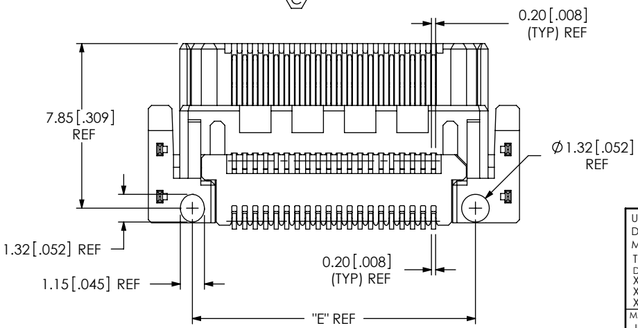
FIG 1 LSHM-120-X1-X-RH-A-N-X-XX SHOWN
