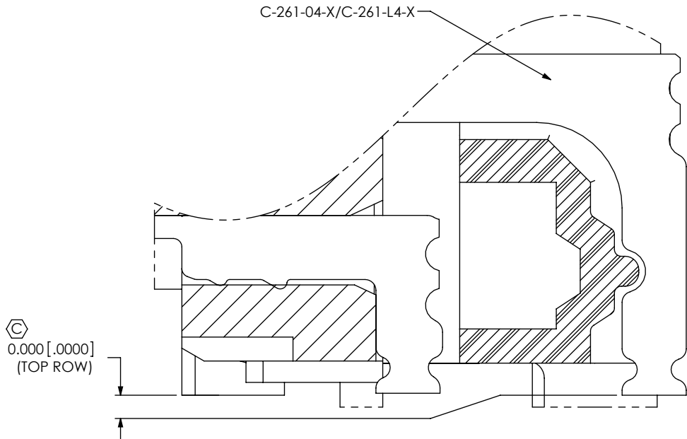
TOP ROW-TAIL DETAIL (LOCATE ASSY ON DATUM -C- FOR MEASUREMENT)
