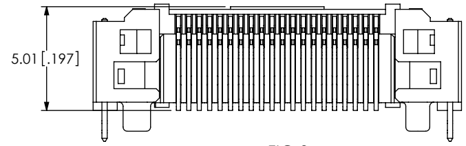
FIG 3 LSHM-120-X1-X-RH-A-N-K-XX SHOWN
