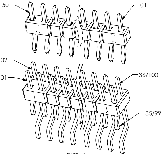
FIG 4 POLARIZATION VIEW
