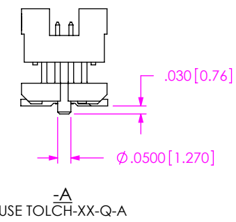
FIG 2 *TOLCH BODY IN THIS DESIGN REFLECTS ALTERNATE STANDOFF DESIGN
